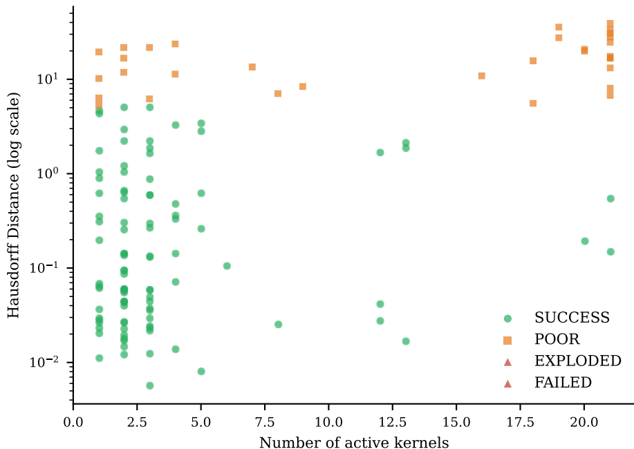
Active kernels vs reconstruction error (130 systems)
