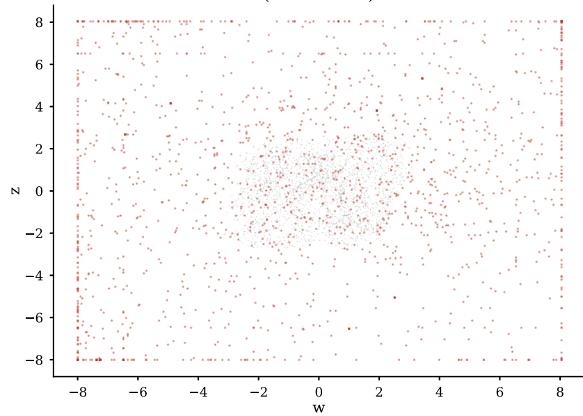
DoublePendulum (HD = 32.894)
