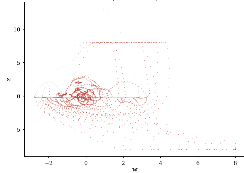
HyperRossler (HD = 21.384)
