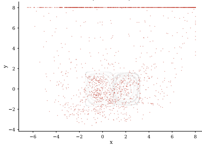
DoubleGyre (HD = 19.658)
