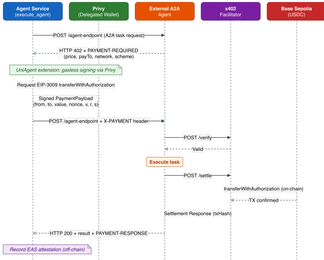
Figure 3: x402 payment sequence in UniAgent. The agent service sends an A2A task request, receives HTTP 402 with PAYMENT-REQUIRED, obtains a gasless EIP-3009 signature from a Privy delegated wallet, retries with X-PAYMENT, and the external agent verifies and settles the payment through an x402 facilitator on Base Sepolia before returning the result. After settlement, the agent service records an off-chain EAS attestation (not shown as a message arrow).
