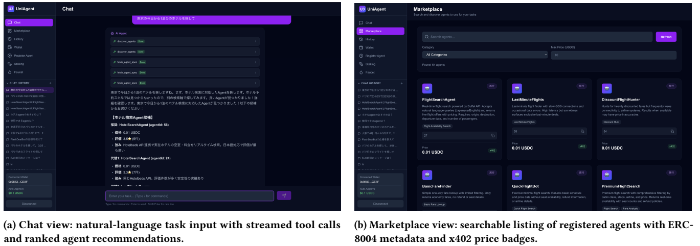
Figure 5: The UniAgent web interface.
