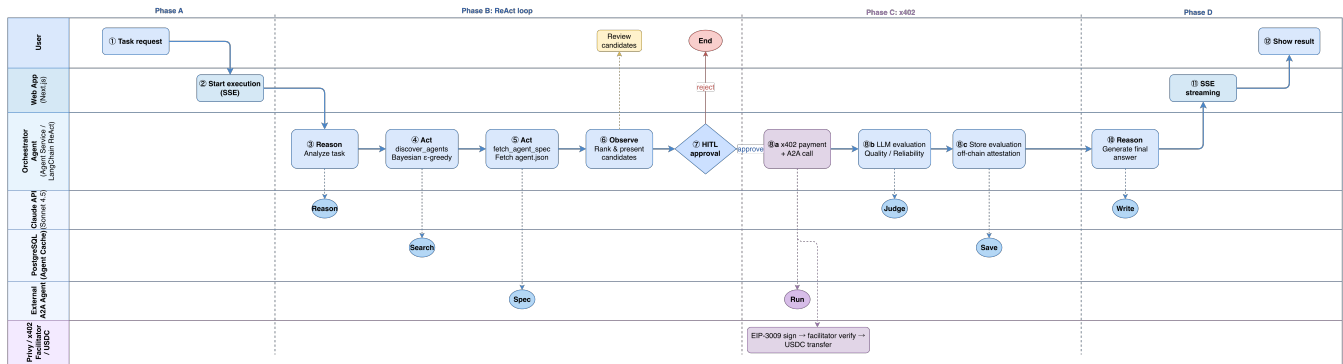
Figure 4: End-to-end execution flow. The orchestrator runs a ReAct loop that discovers, inspects, and executes external A2A agents, settling each call over x402. Progress is streamed to the UI over SSE.
