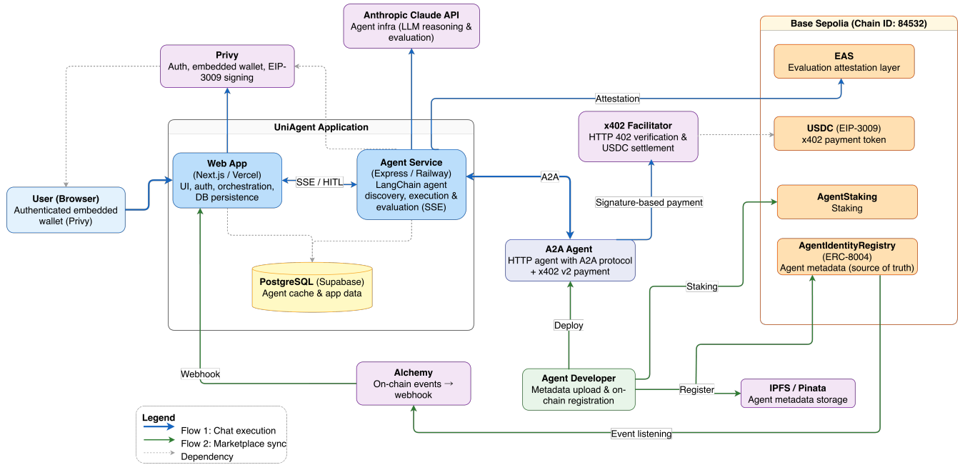
Figure 1: Overview of the UniAgent architecture. A user issues a natural-language task through the web application; an LLM-based agent service discovers candidate agents from an ERC-8004 registry (cached in PostgreSQL via Alchemy webhooks), invokes the selected external A2A agents, and settles payment over x402 using USDC on Base Sepolia.
