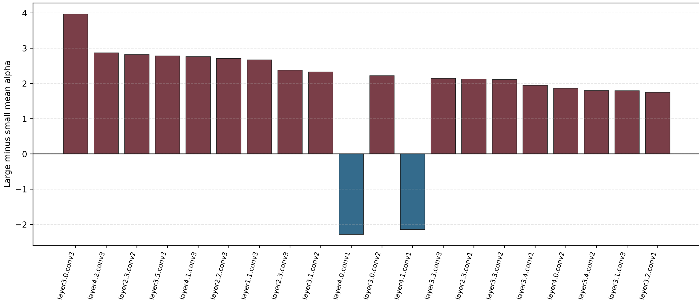
Layerwise alpha gap: large-data vs small-data source models
