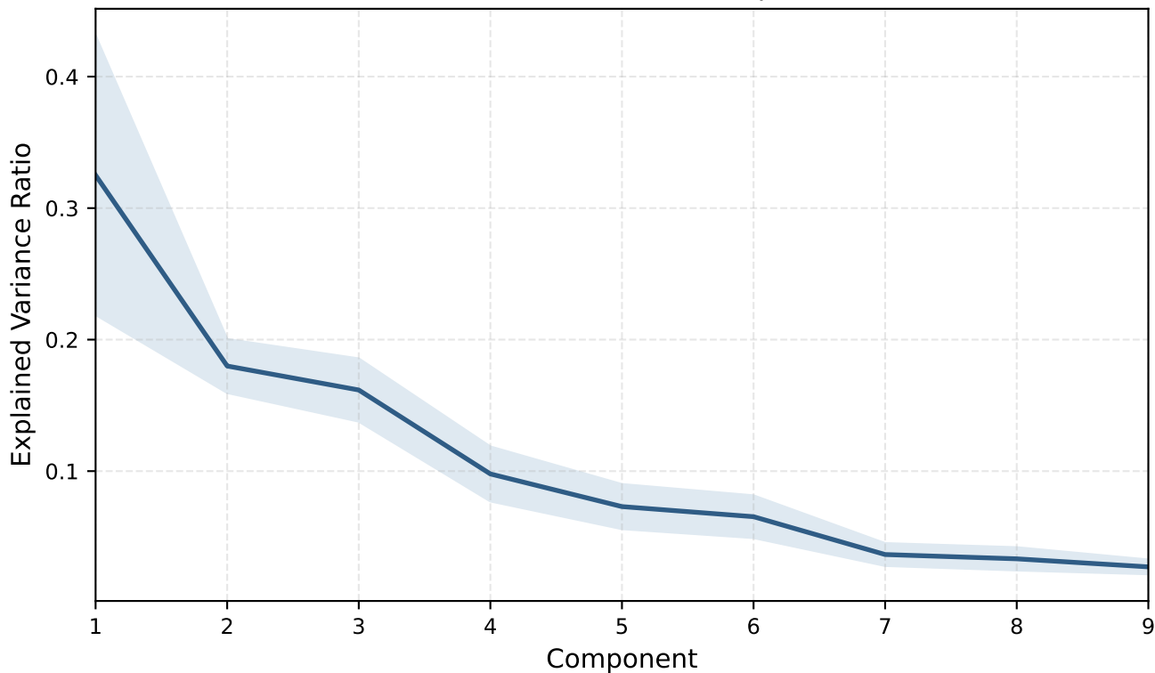
Mean scree across shared ResNet50 spatial kernel bases
