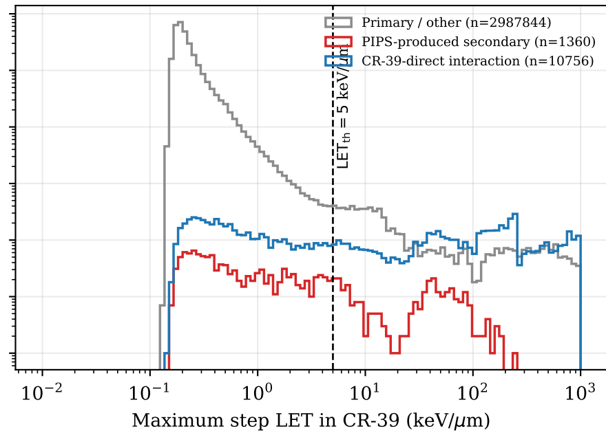
Pions/kaons/protons, 10 GeV/c
