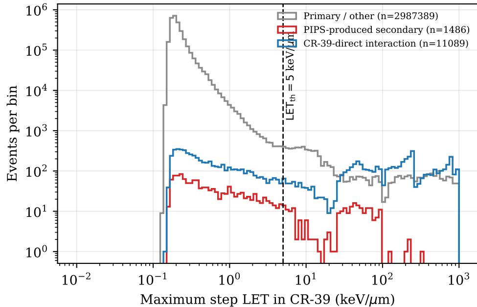
Pions/kaons/protons, 4.5 GeV/c
