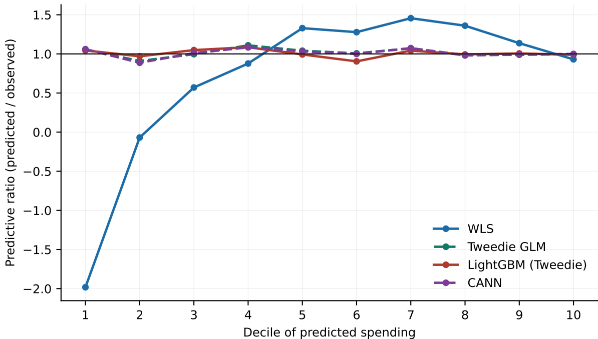
Calibration across the distribution of predicted spending
