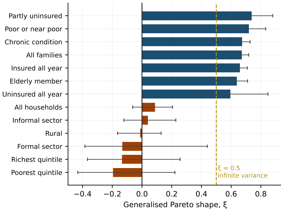
Tail heaviness
