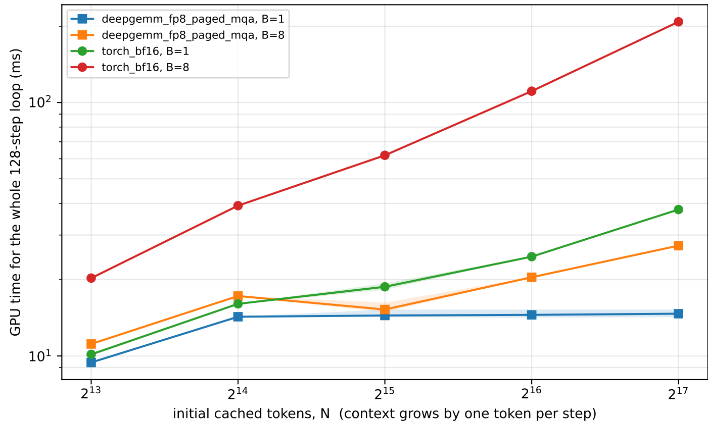
DSA incremental decode: append one indexer key + search, 128 steps context length grows within each measured loop
