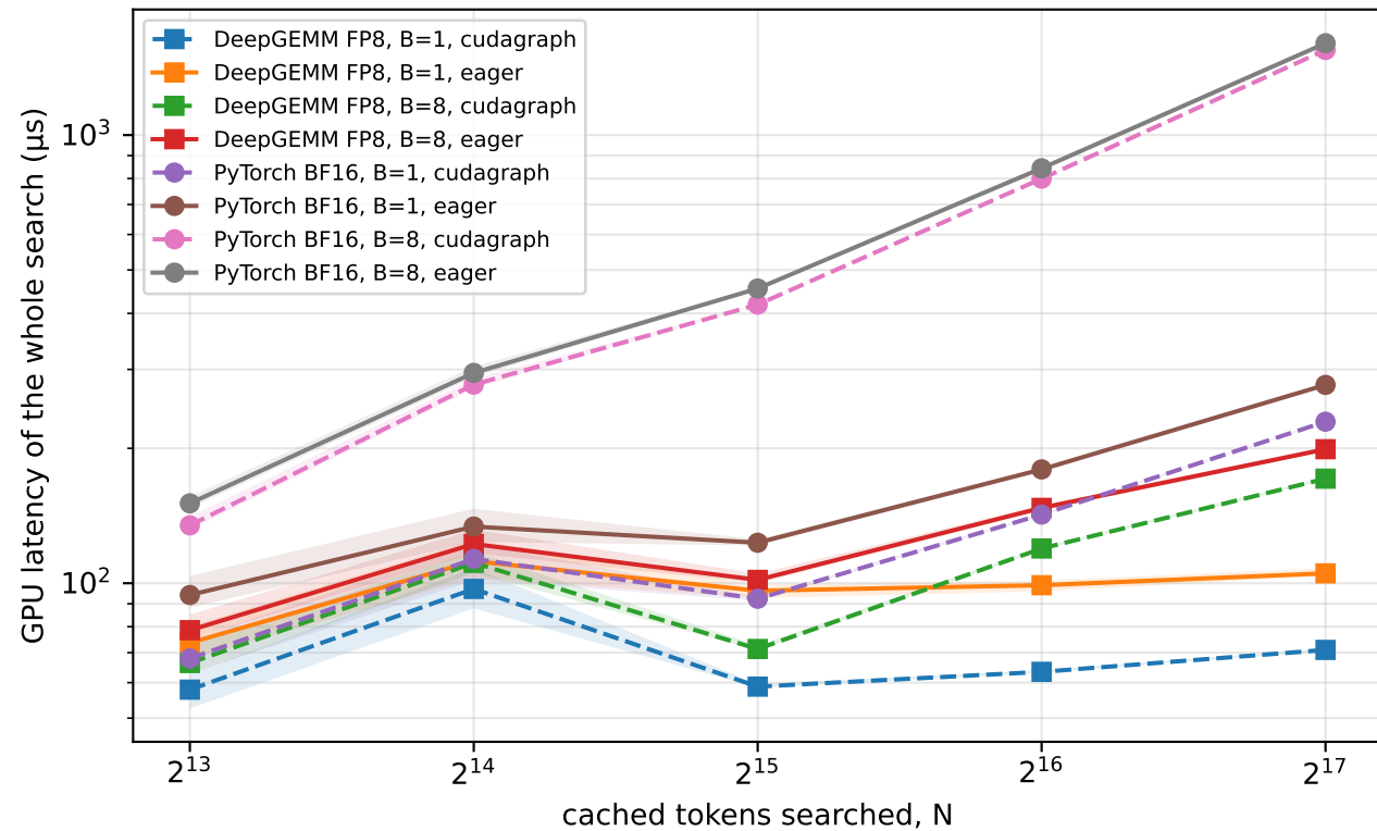
DSA indexer search score + top-k, one timed operation
