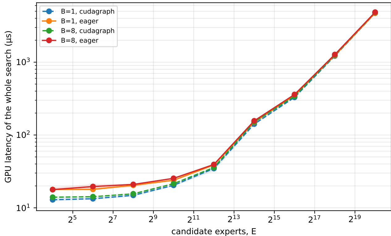
Flat MoE router search score + top-k, one timed operation
