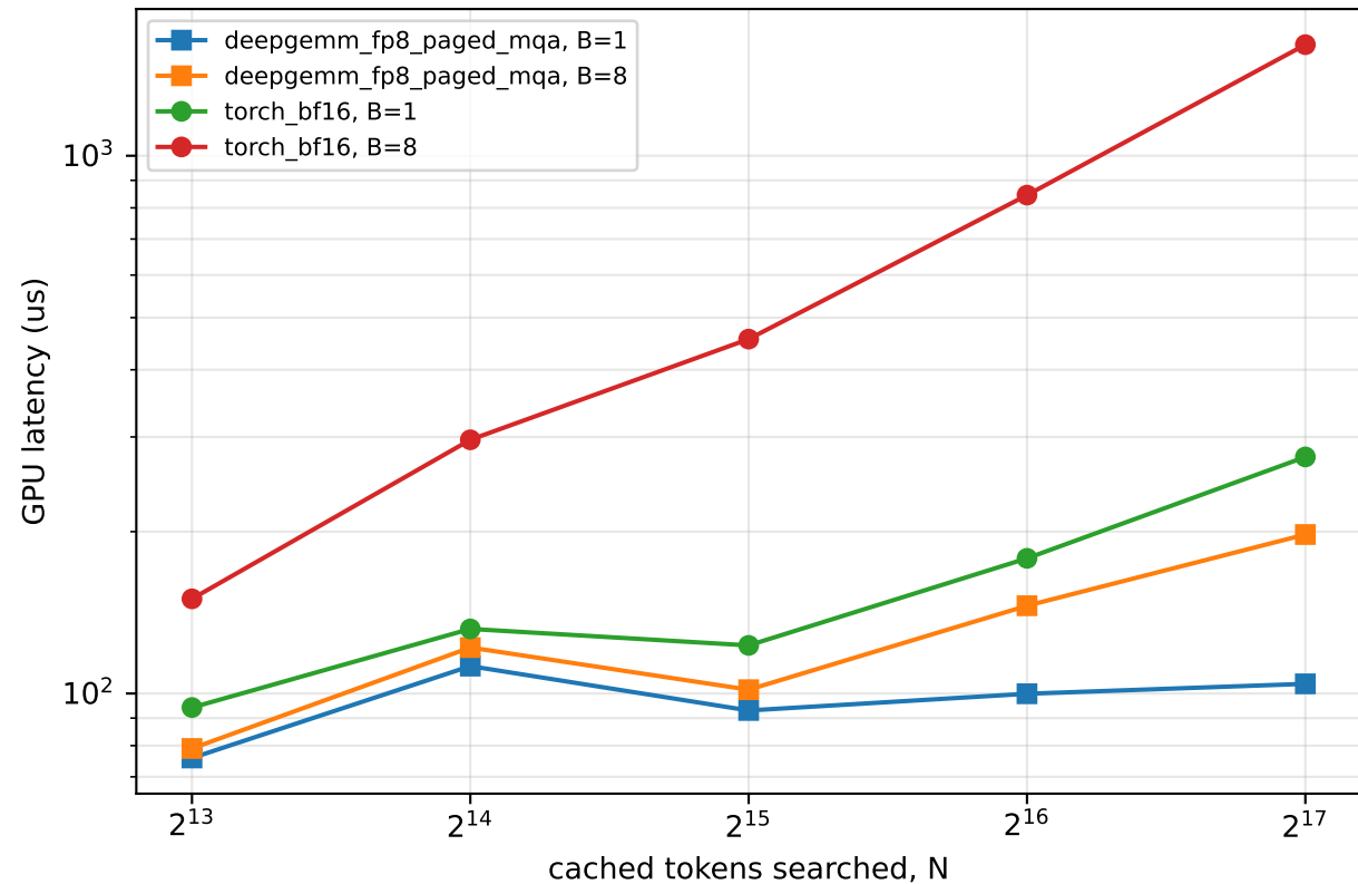
Combined DSA search (scoring + top-k)
