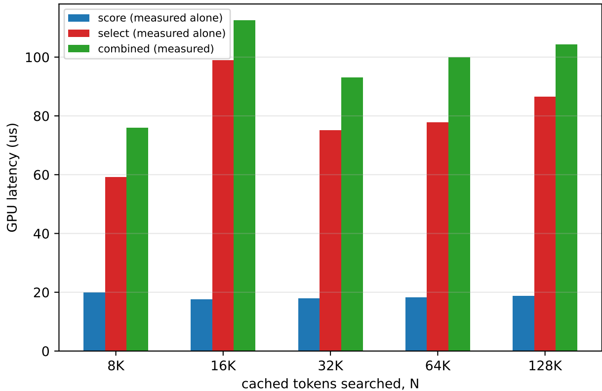
deepgemm_fp8_paged_mqa, B=1: stages measured side by side (grouped, not stacked - stages need not sum)
