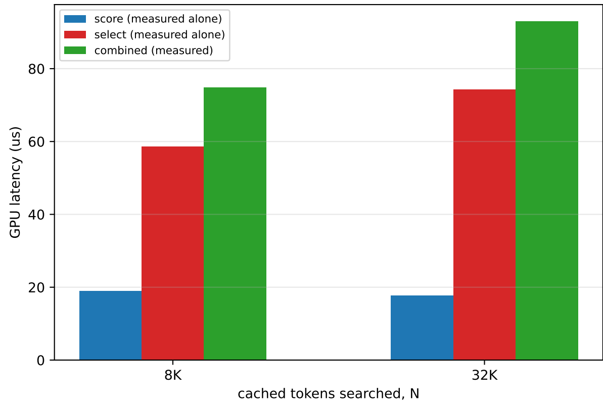
deepgemm_fp8_paged_mqa, B=1: stages measured side by side (grouped, not stacked - stages need not sum)
