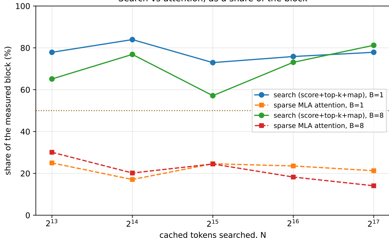
Search vs attention, as a share of the block
