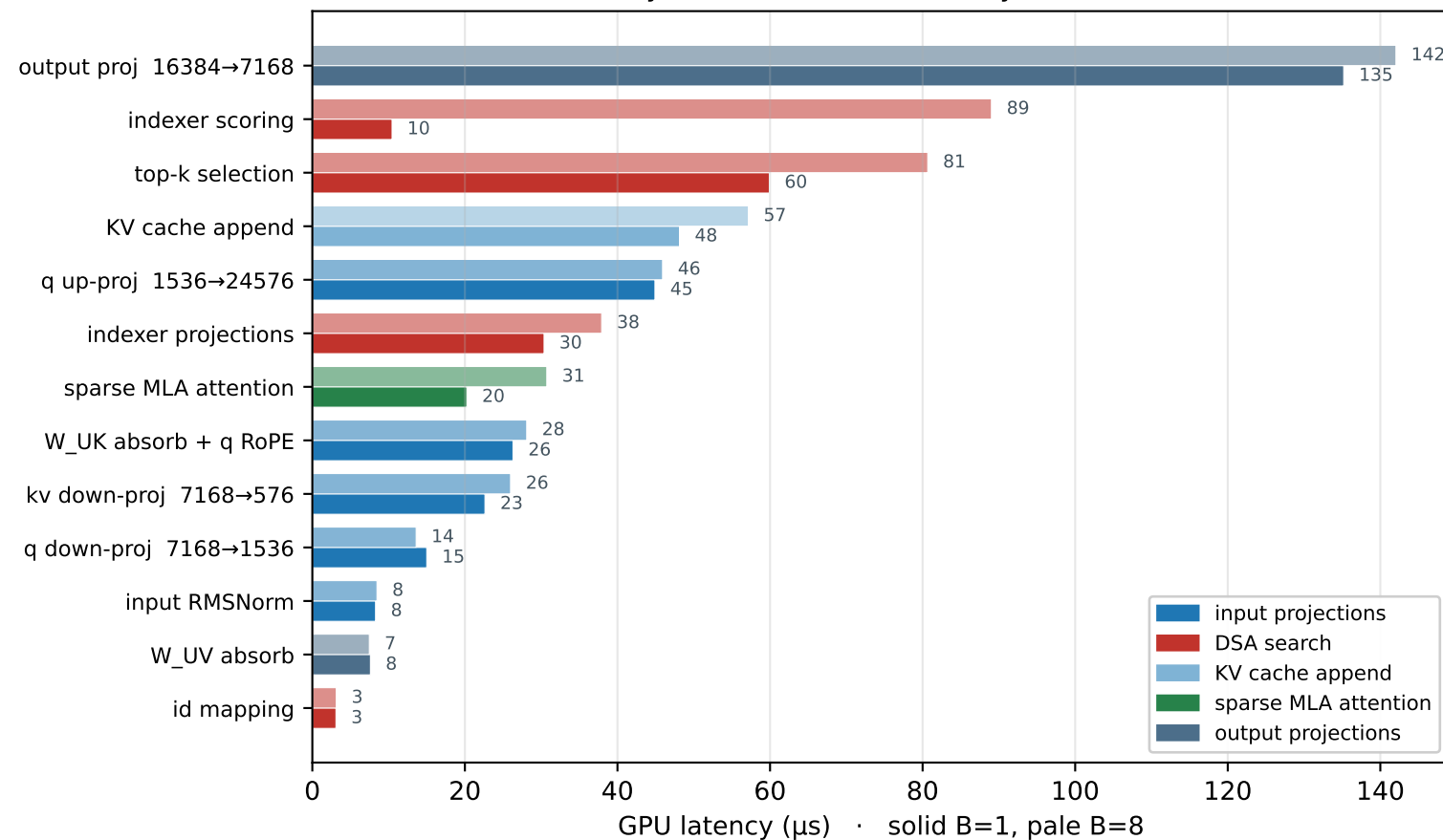
Every block of the MLA sub-layer, N=128K
