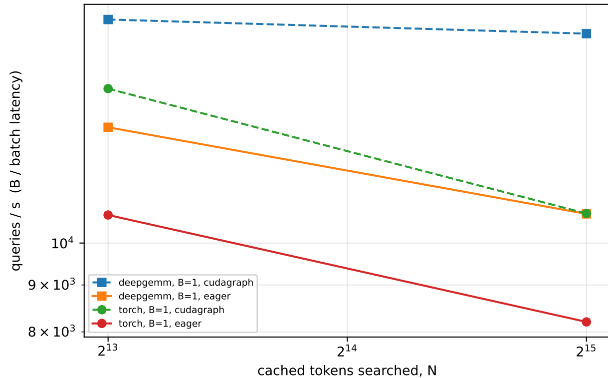
DSA search throughput
