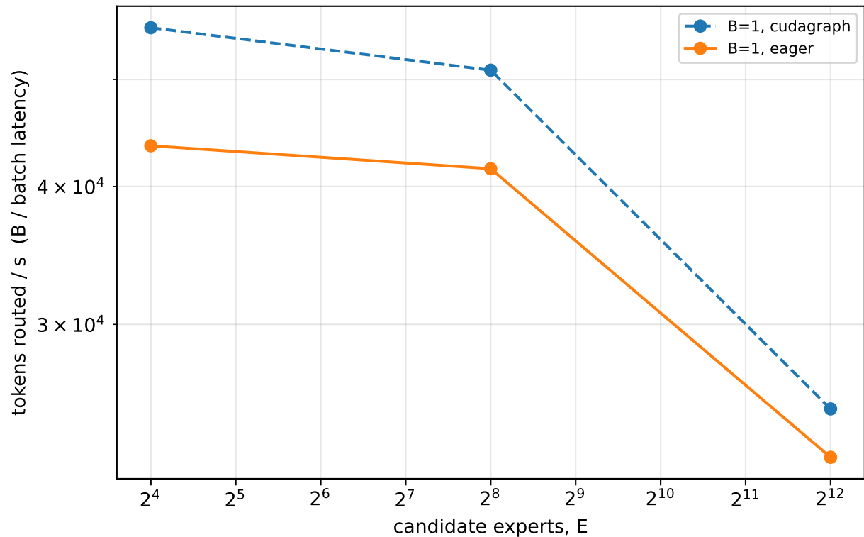
Router throughput
