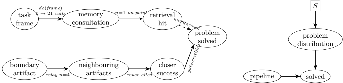
Figure 1: Left: the mechanism DAG as currently witnessed. Solid edges carry certificates (labels); the dashed edge is the honest gap — retrieval hits have not yet been shown to cause solutions (every hint so far was correctly discarded as off-route). The do ( \cdot ) edge is the programme’s one true intervention: a preregistered controlled contrast on the task frame. The lower path is the relay: boundary artifacts and neighbouring solved problems feed closer success ( n=4 witnessed hops), which the mechanical gate certifies into solutions. Right: the transport question N6 as a selection diagram: S switches the problem distribution (APM vs. held-out BPM); “the pipeline works on BPM” is identified only if the S -dependence can be separated from the pipeline edge — a derivation obligation, not an extrapolation.
