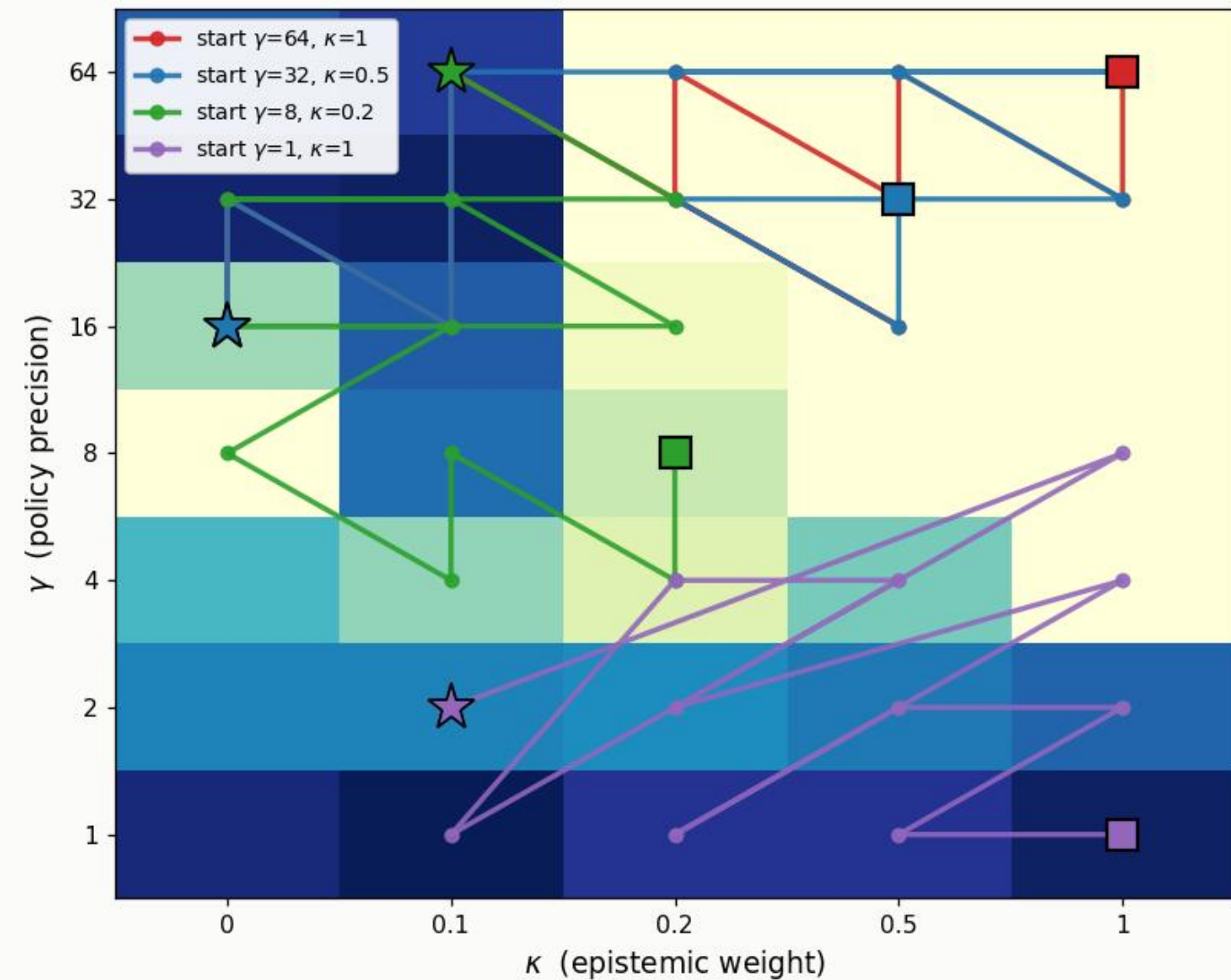
control space — objective surface + search paths
