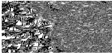
The found configuration: structured and chaotic regimes side by side—Fig. 14, ⟨1.3.2⟩
