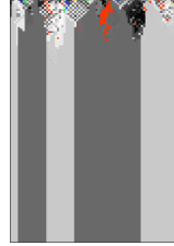
Dead genotype, live phenotype at \lambda = \frac{1}{2} —Fig. 4,
