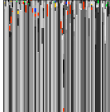
Even cycles: fixed point exists, field settles—Fig. 5,
