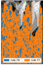
The 2015 operator collapses its genotype—Fig. 2, ⟨1.1.1⟩
