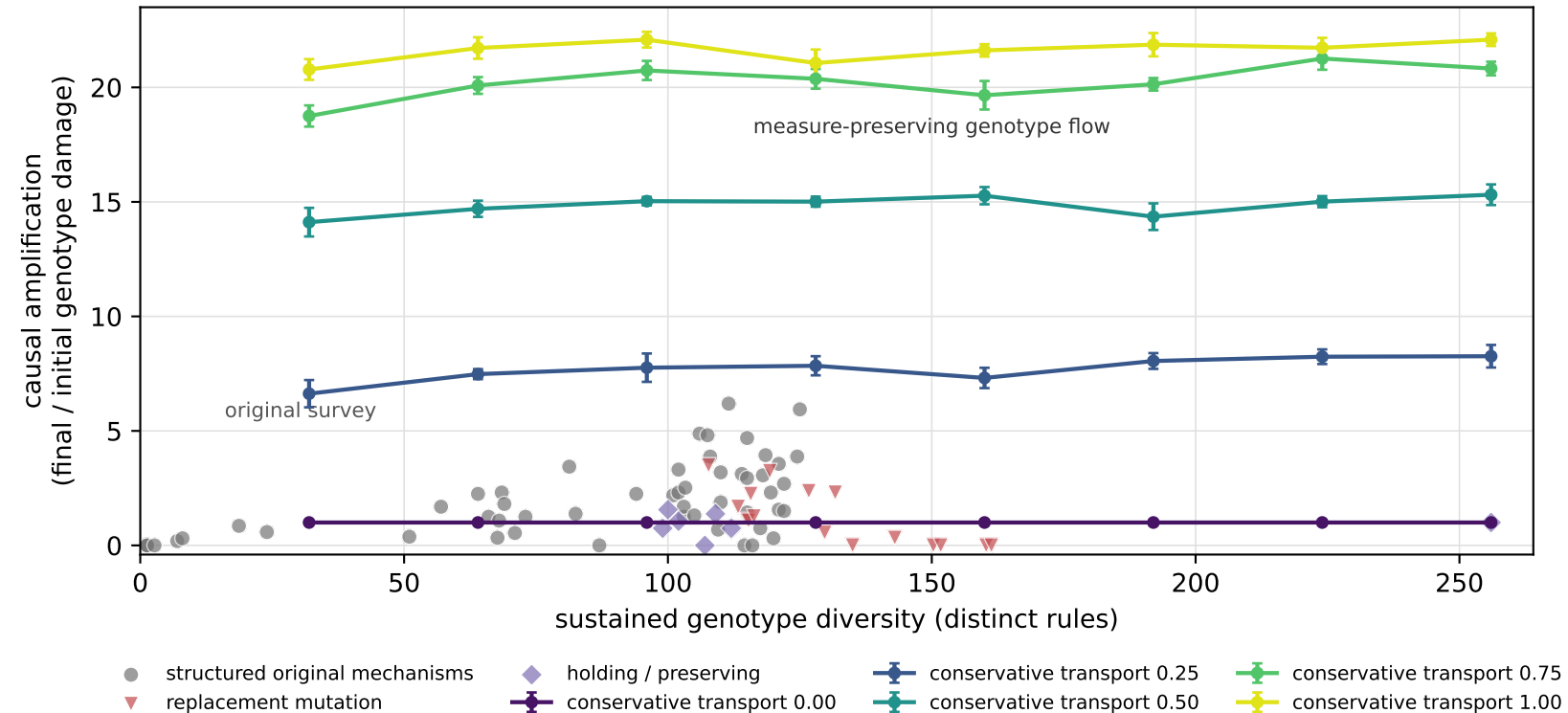
Causal amplification depends on conservative transport, not diversity alone
