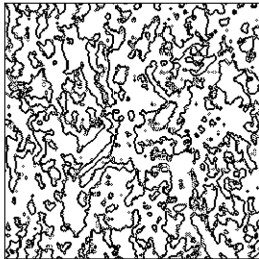
river: D=1.80
