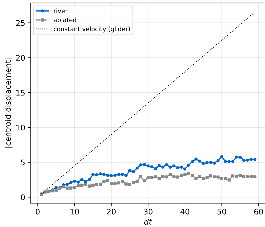
(b) centroid wanders ( \sim dt^{0.56} ), does not translate
