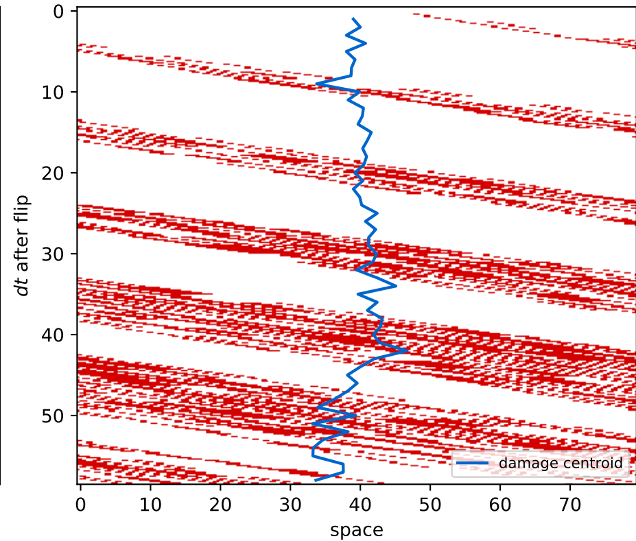
(c) one cone: the centroid drifts, the packet disperses
