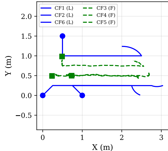
(a) Desired Trajectories
