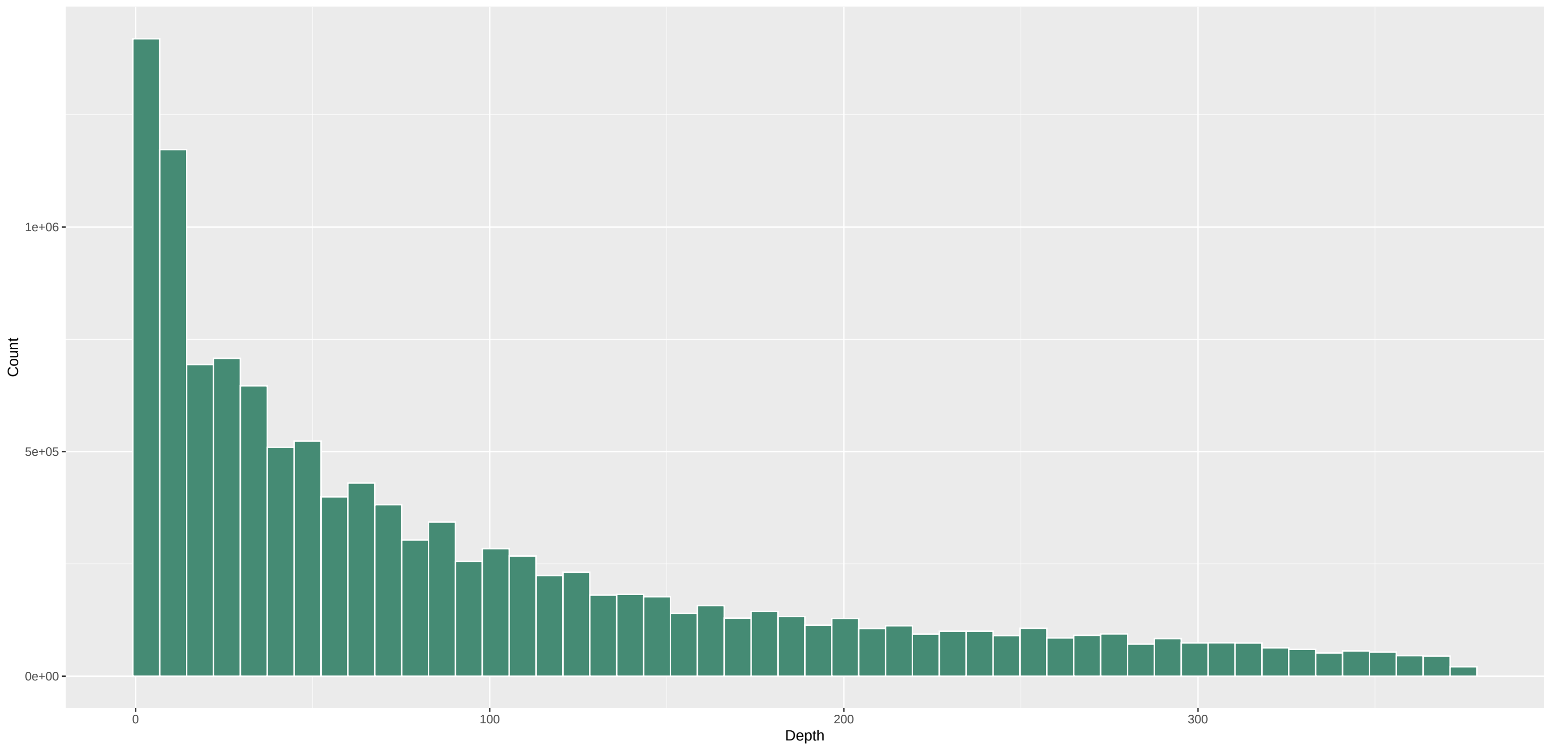
DP distribution (full data) – Vill.C6.3
