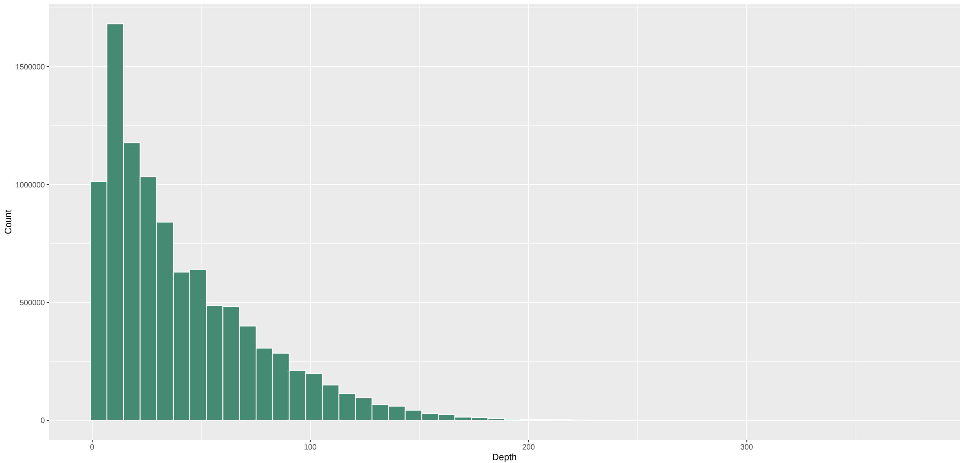
DP distribution (full data) – Vill.C19.1
