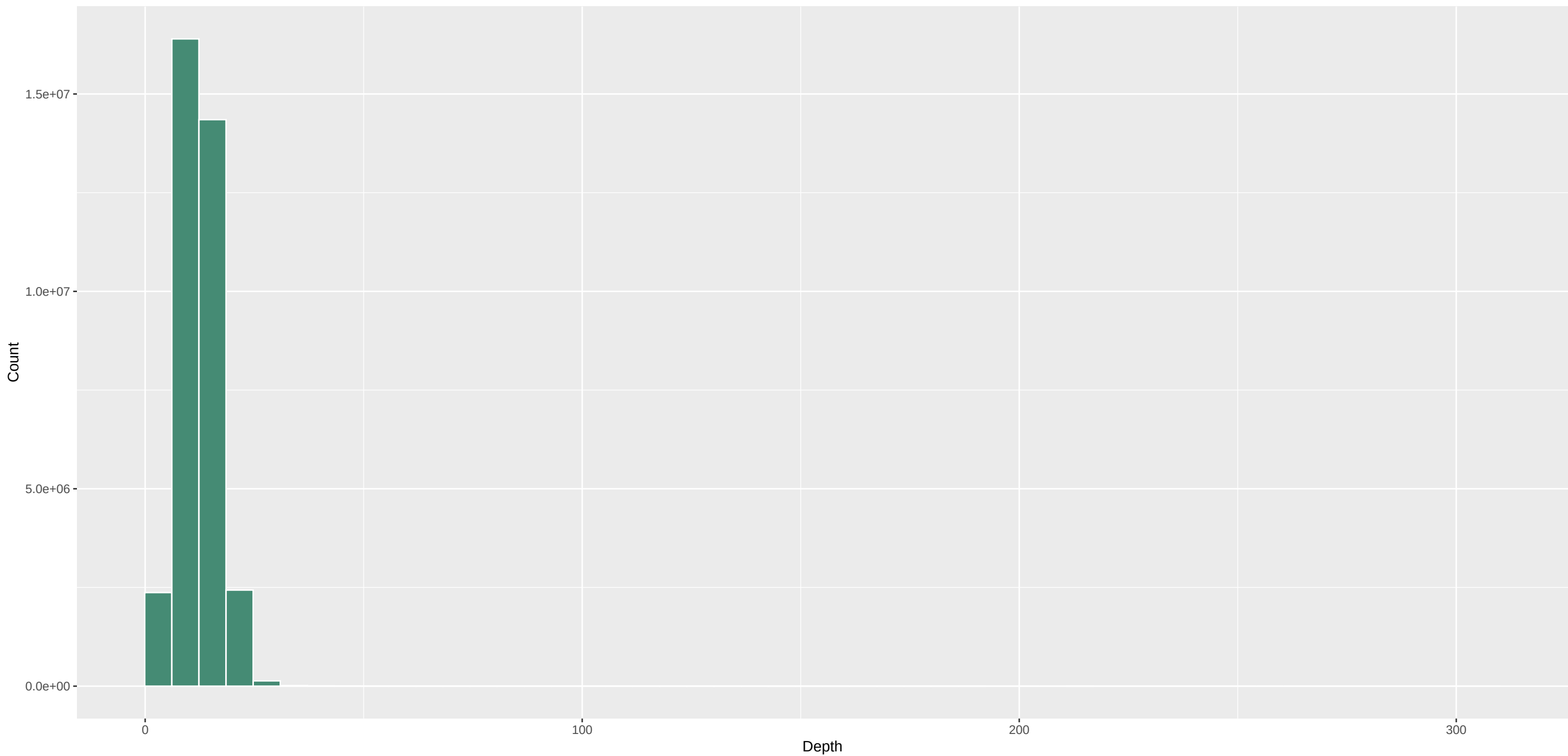
DP distribution (full data) – Vill-A1-2_S63
