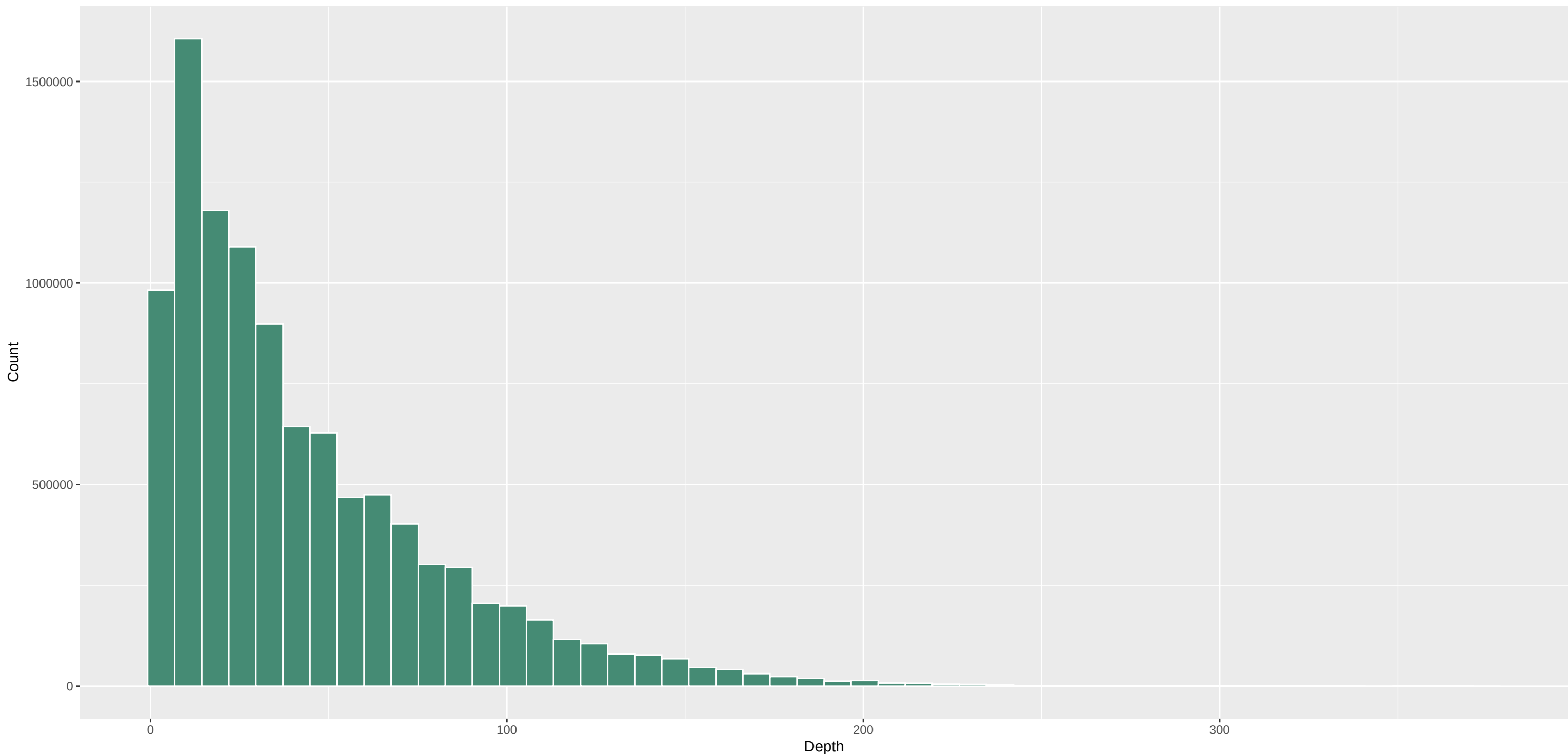
DP distribution (full data) – Vill.C8.1
