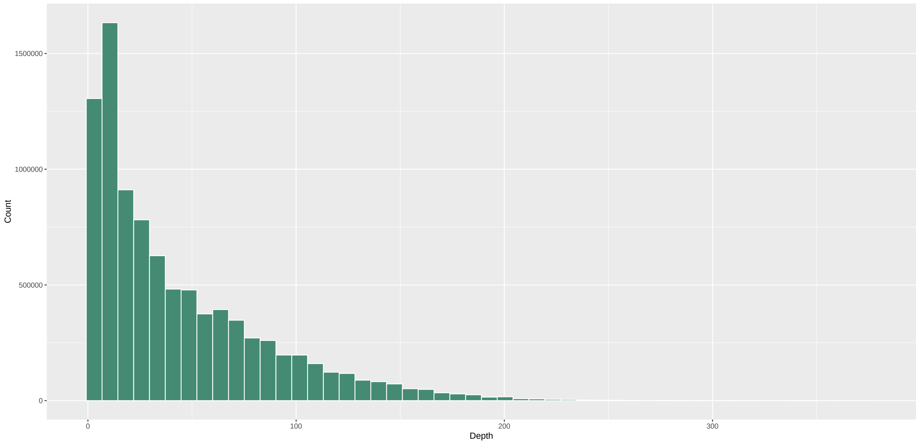
DP distribution (full data) – Vill.C6.5
