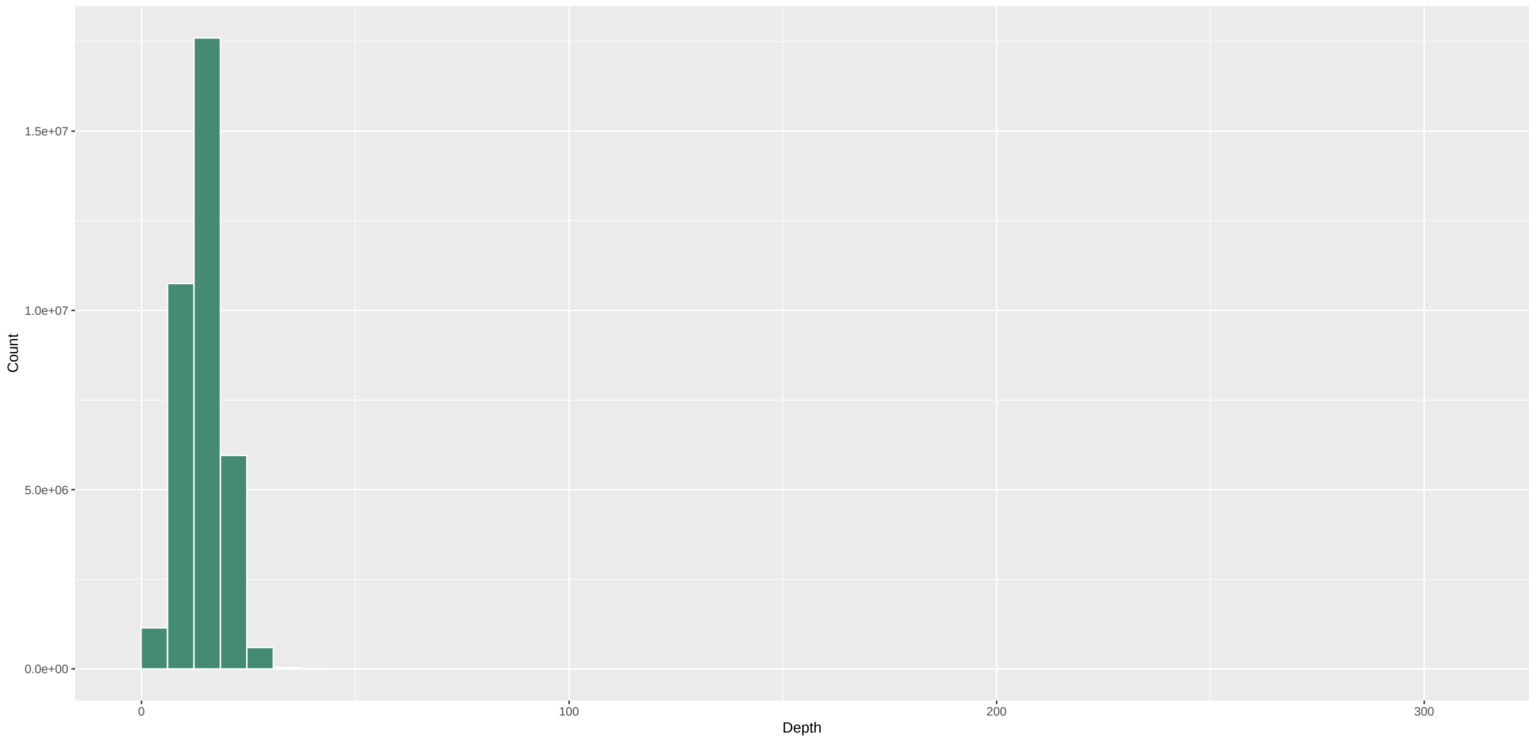
DP distribution (full data) – Vill-A1-3_S79
