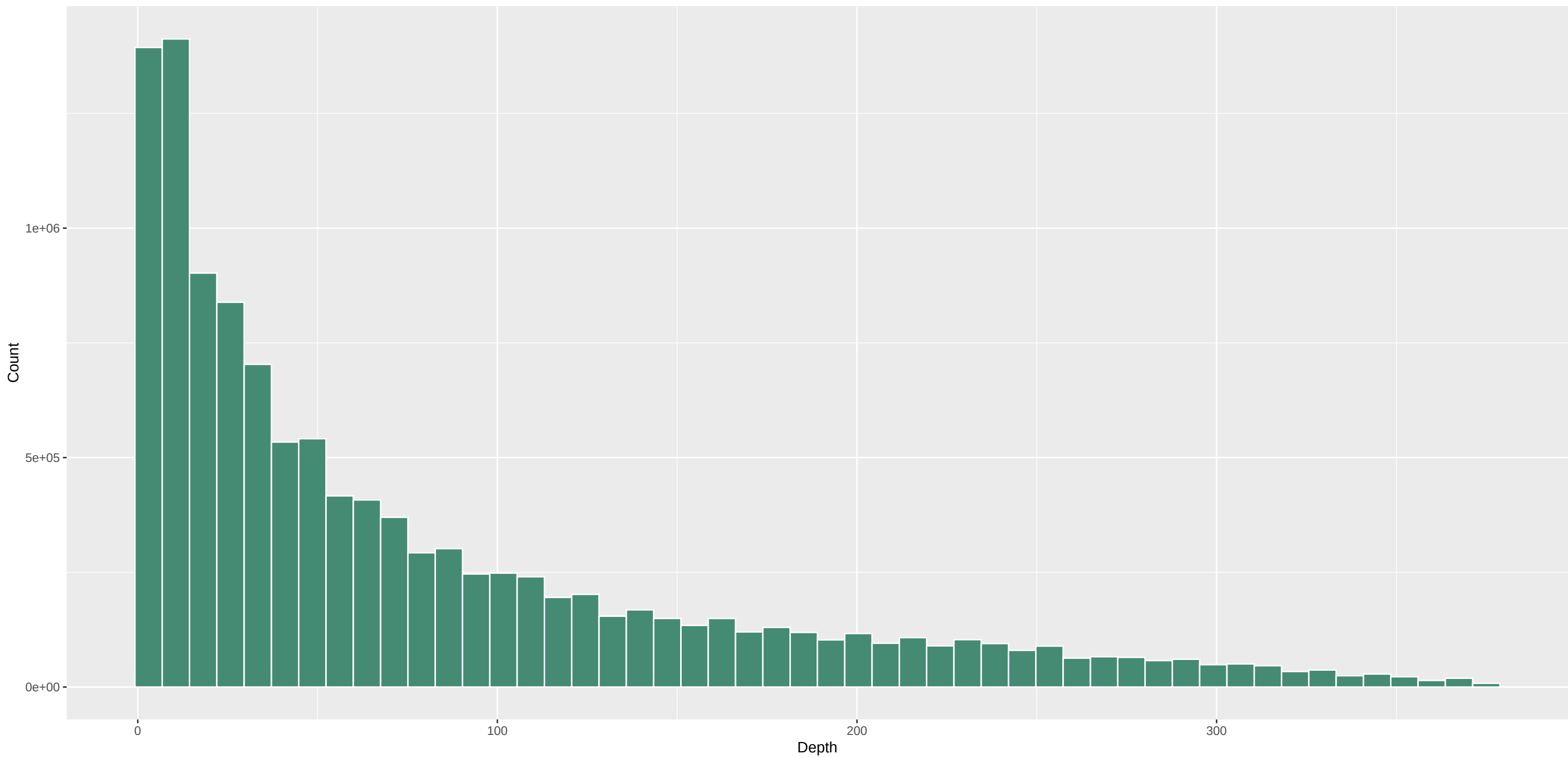
DP distribution (full data) – Vill.C1.1BIS
