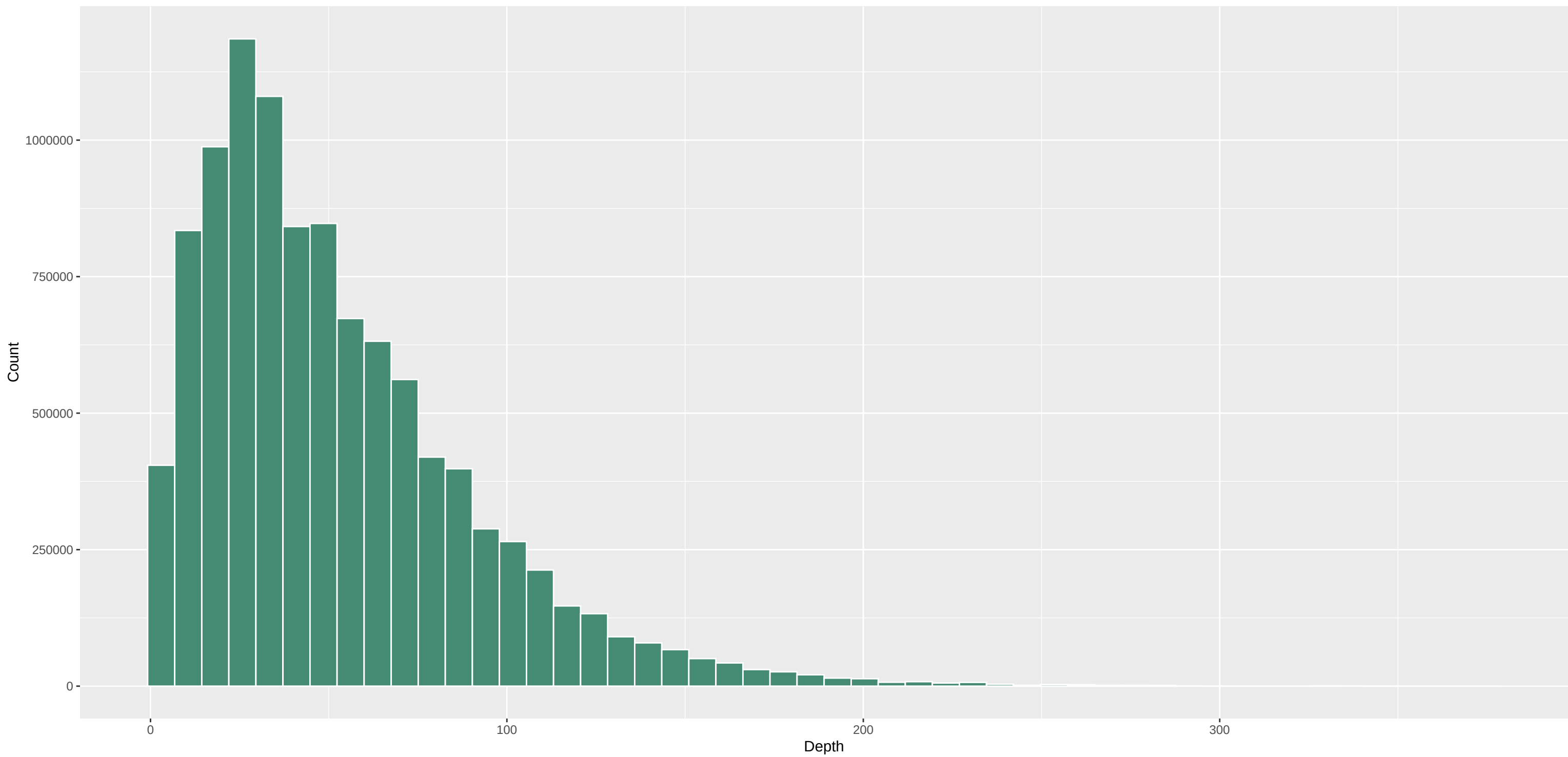
DP distribution (full data) – Vill.C31.1
