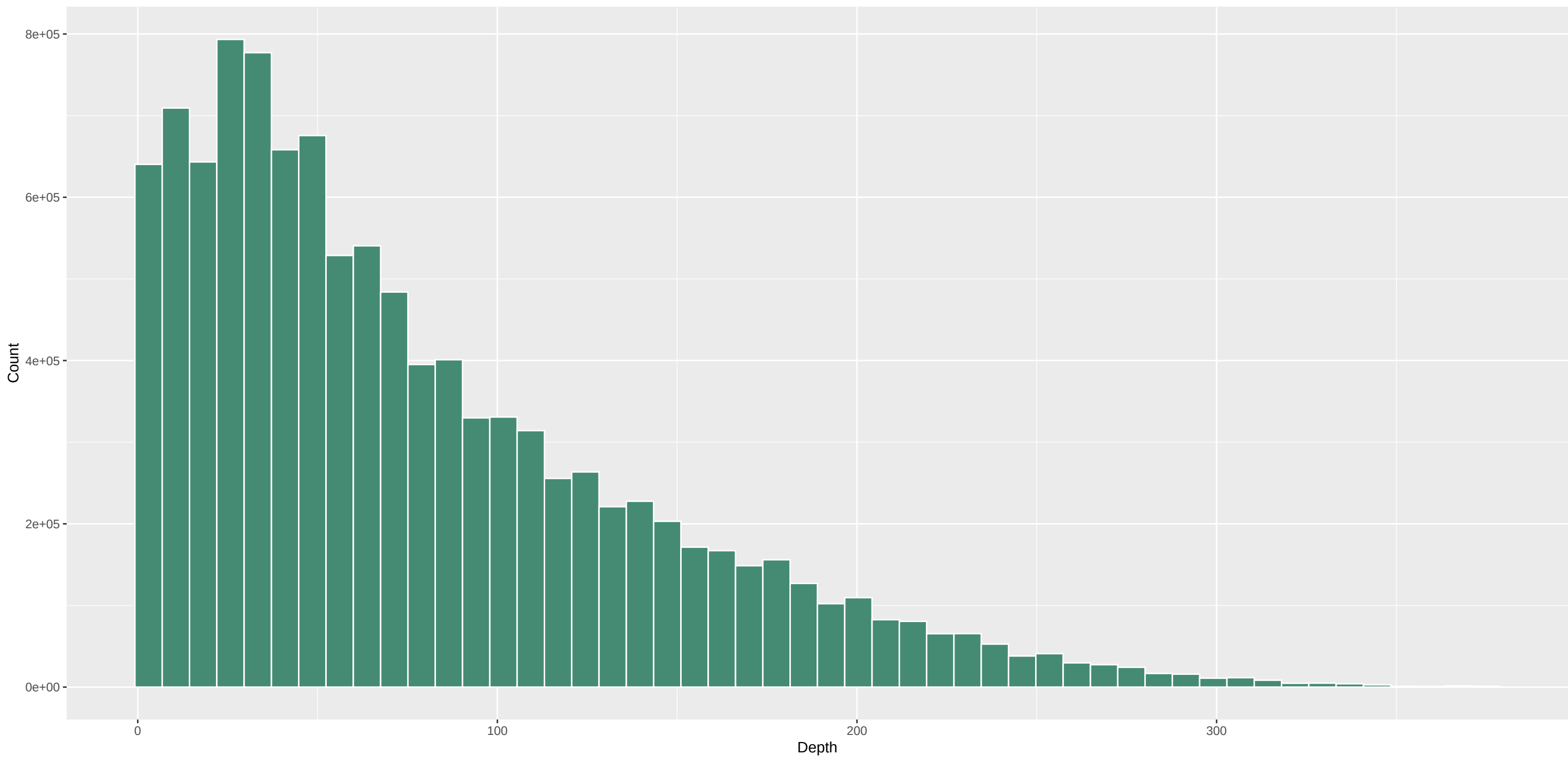
DP distribution (full data) – Vill.C2.2
