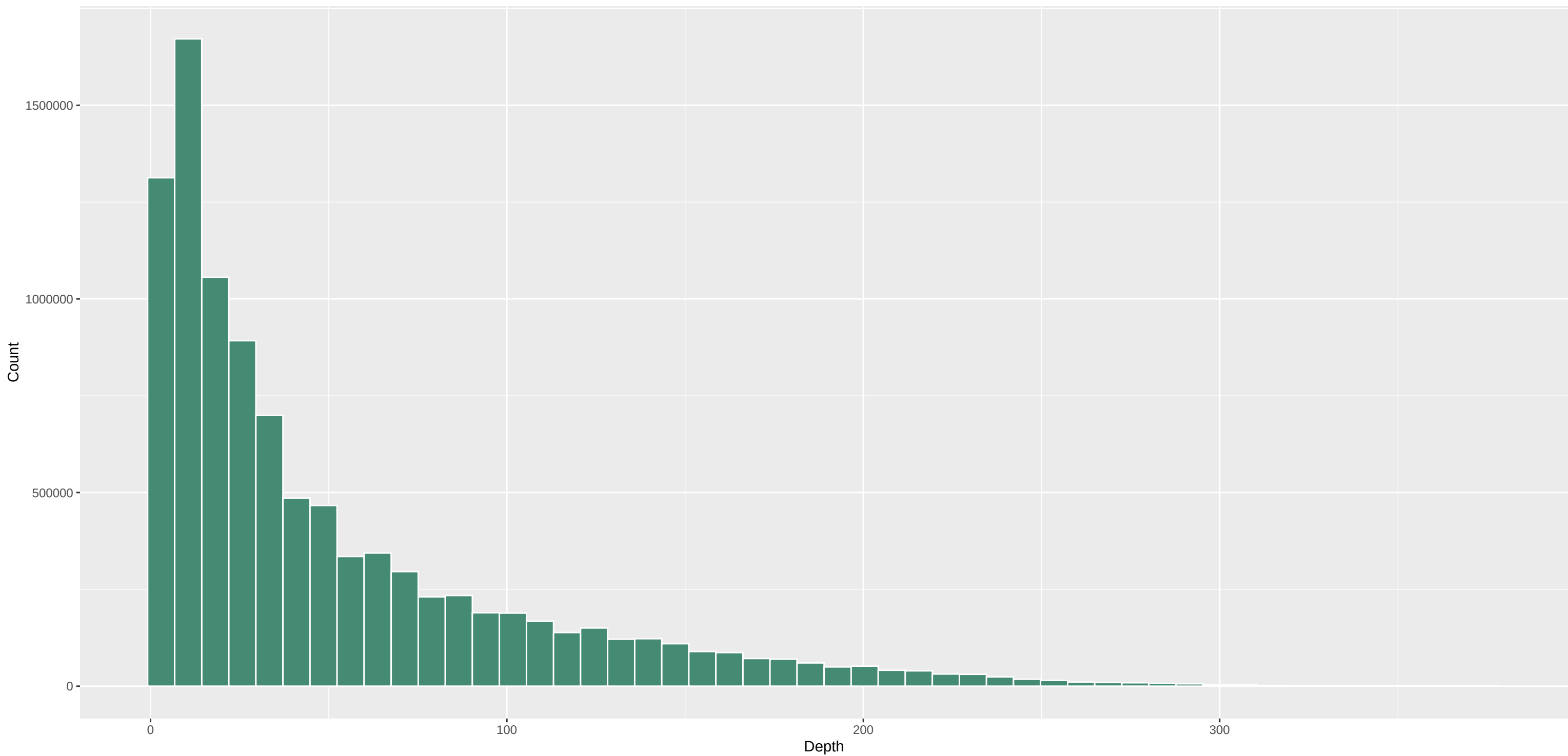
DP distribution (full data) – Vill.C28.1
