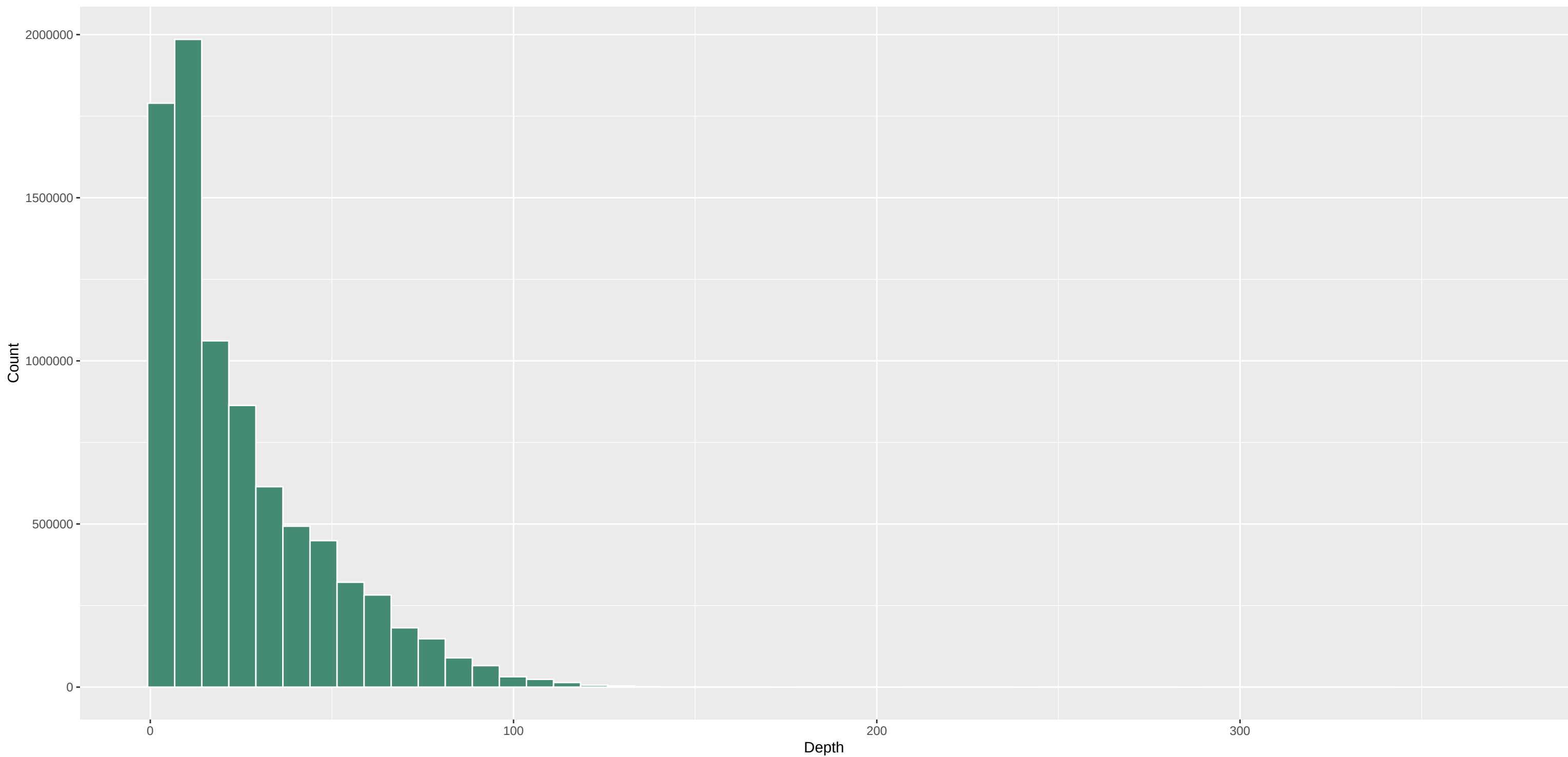
DP distribution (full data) – Vill.C21.1
