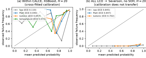
Fig. 3. Reliability diagrams under the cross-fitted protocol. (a) Within CALCE (XGBoost, H=20 ). (b) ALL-LCO→Severson without SOH ( H=20 ): no source-fitted calibrator lands near the diagonal on the shifted target.
