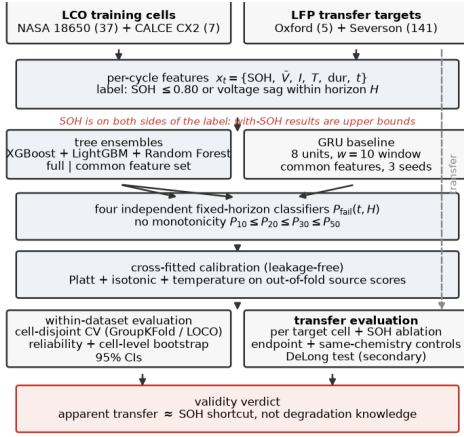
Fig. 1. Overview of the proposed multi-horizon failure-risk framework: datasets, features and labels, model families, per-horizon classifiers, cross-fitted calibration, and the reliability, transfer, and shortcut-control evaluations.
