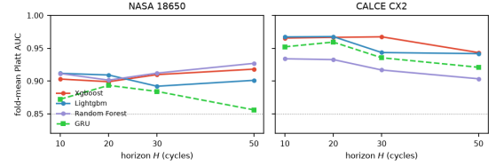
Fig. 2. Within-dataset fold-mean Platt AUC across prediction horizons (NASA and CALCE, cell-disjoint CV).
