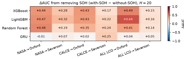
Fig. 4. Transferability collapse map at H=20 : AUC drop from removing SOH, per source→target pair and model.
