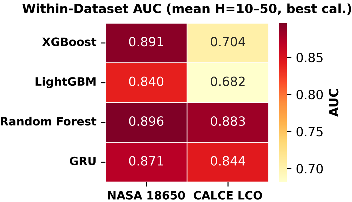
FIGURE 2. Within-dataset AUC heatmap, mean across horizons, Platt-calibrated.
