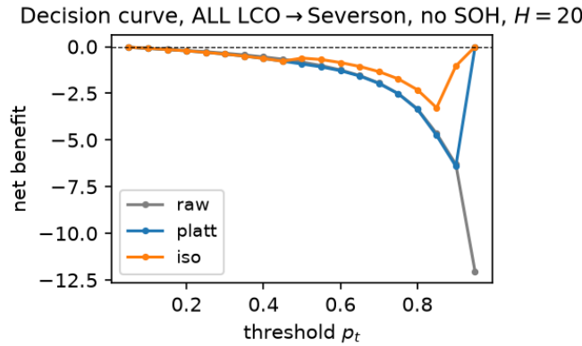
FIGURE 5. Decision-curve analysis (net benefit vs. threshold) for ALL-LCO → Severson without SOH at H=20 : no score type produces a usable operating point once SOH is removed.
