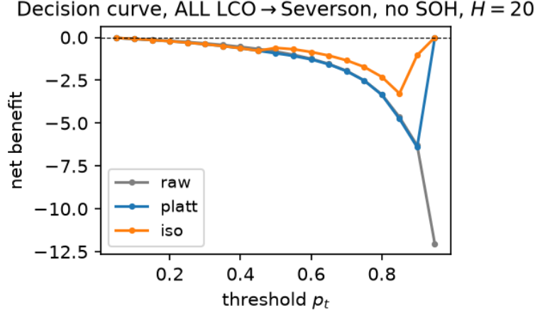
Figure 5: Decision-curve analysis (net benefit vs. threshold) for ALL-LCO → Severson without SOH at H=20 : no score type produces a usable operating point once SOH is removed.
