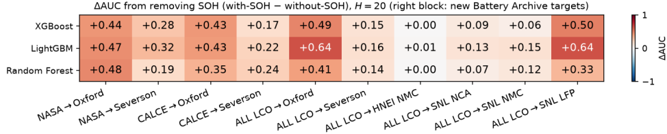
Figure 2: Transferability collapse map at H=20 for the tree ensembles: the AUC drop from removing SOH, per source→target pair and model. Positive values mean SOH removal destroys apparent transfer performance; the near-uniform saturation at the maximum drop is the signature of a single-feature shortcut rather than of distributed degradation knowledge. Right block: ALL-LCO → new Battery Archive targets. GRU deltas are reported in the text.
