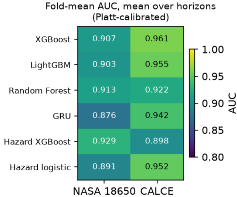
FIGURE 2. Within-dataset AUC heatmap, mean across horizons, Platt-calibrated.
