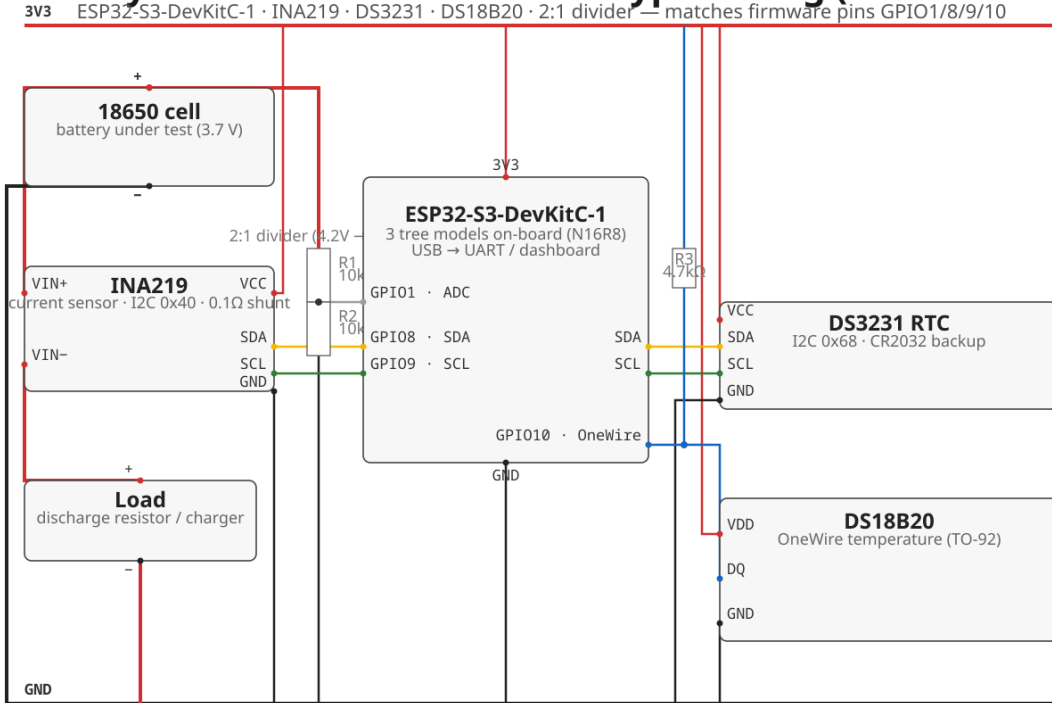
FIGURE 1. Prototype wiring for the ESP32-S3 deployment. The battery discharges through the INA219 shunt into a load, the 2:1 divider senses cell voltage at ADC GPIO1, and I2C (GPIO8/9) serves the INA219 and DS3231 while OneWire (GPIO10) reads the DS18B20. The boards are a $12 ESP32-S3-DevKitC-1 and two breakout modules.
