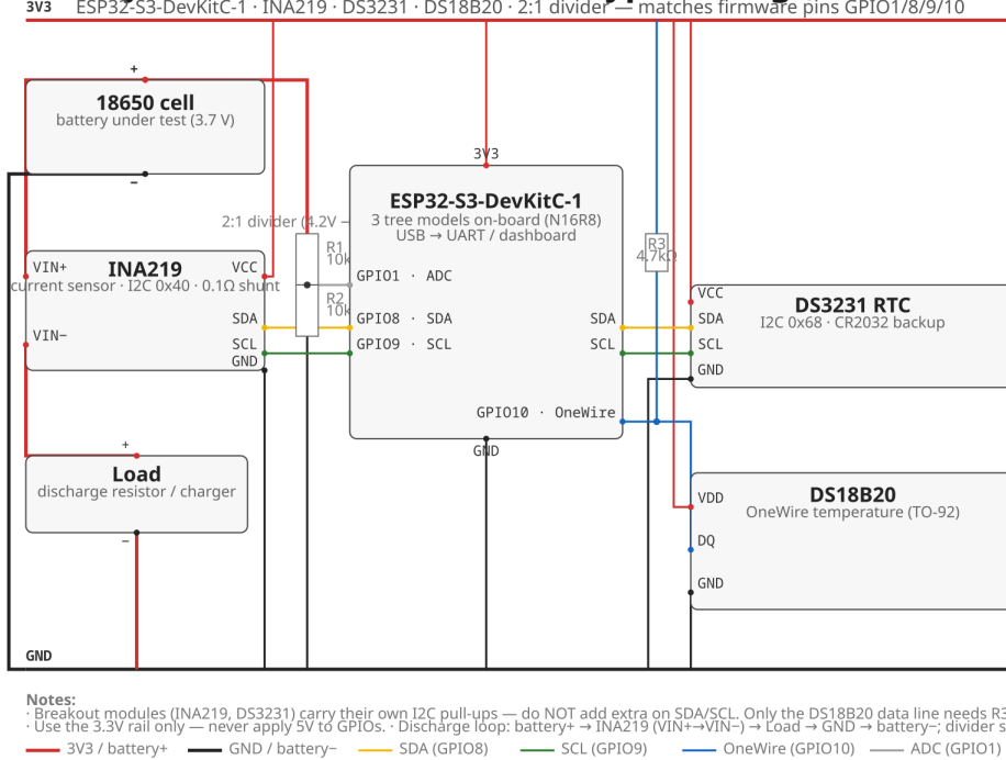
FIGURE 1. Prototype wiring for the ESP32-S3 deployment. The battery discharges through the INA219 shunt into a load, the 2:1 divider senses cell voltage at ADC GPIO1, and I2C (GPIO8/9) serves the INA219 and DS3231 while OneWire (GPIO10) reads the DS18B20. The boards are a $12 ESP32-S3-DevKitC-1 and two breakout modules.
