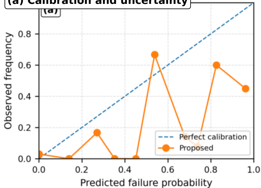
(a) Calibration and uncertainty
