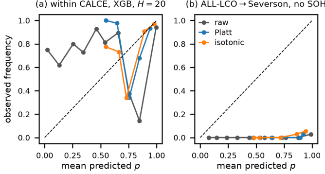
Fig. 3. Reliability diagrams under the cross-fitted protocol. (a) Within CALCE. (b) ALL-LCO→Severson without SOH.
