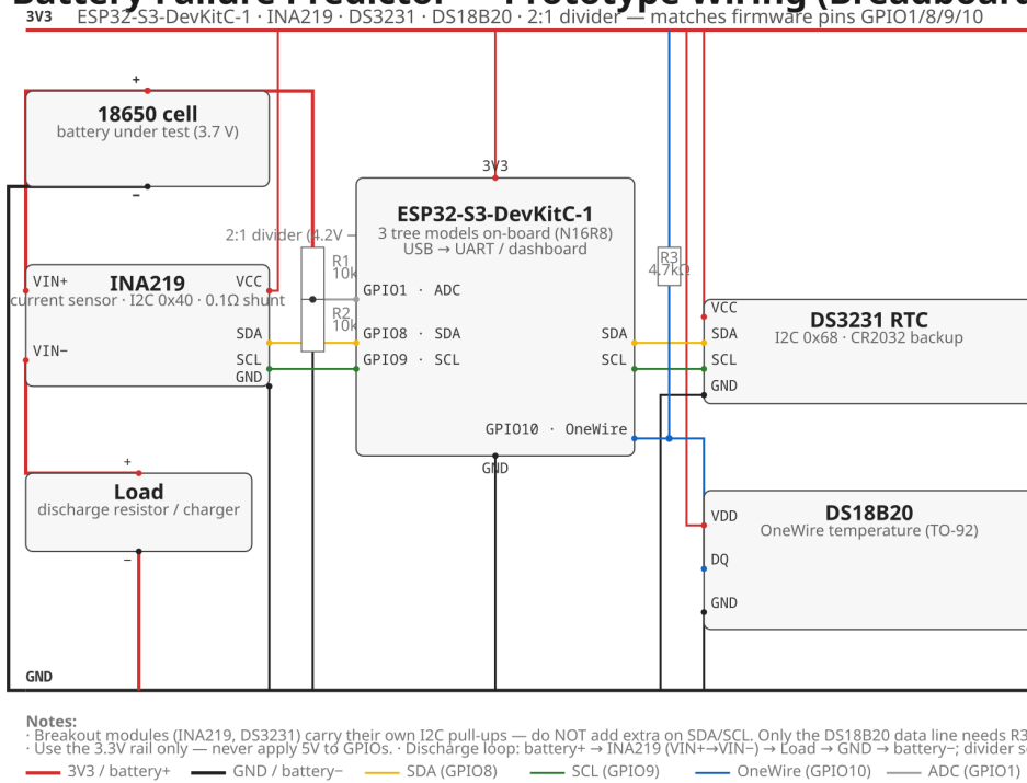
Fig. 1. Prototype wiring for the ESP32-S3 deployment. The battery discharges through the INA219 shunt into a load, the 2:1 divider senses cell voltage at ADC GPIO1, and I2C (GPIO8/9) serves the INA219 and DS3231 while OneWire (GPIO10) reads the DS18B20. The boards are a $12 ESP32-S3-DevKitC-1 and two breakout modules.
