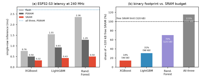
Fig. 12. Deployment trade-offs: (a) measured single-row inference time per model at 240 MHz (PC, and ESP32-S3 with the binary in flash, PSRAM, or a single model in internal SRAM); (b) memory footprint of the 372 kB binary as a share of each tier, exceeding the ESP32-S3's roughly 320 kB of free internal SRAM.
