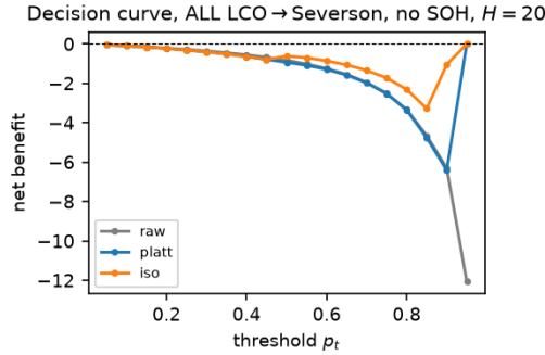
Figure 5: Decision-curve analysis (net benefit vs. threshold) for ALL-LCO \rightarrow Severson without SOH at H=20 : no score type produces a usable operating point once SOH is removed.
