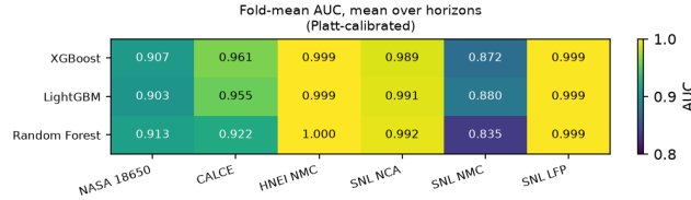
Figure 1: Within-dataset AUC heatmap for the tree ensembles, mean across horizons, Platt-calibrated. Right block: the four new Battery Archive groups. GRU and hazard within-dataset numbers are in Table 2.
