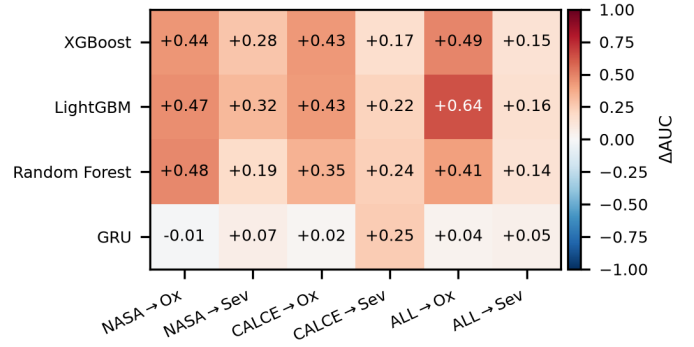
Fig. 4. Transferability collapse map at H=20 .
