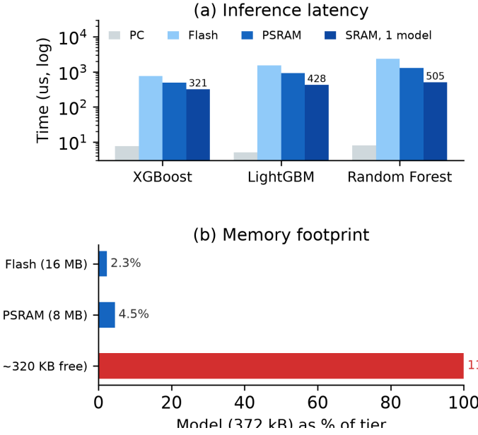
Fig. 12. Deployment trade-offs: (a) measured single-row inference time per model at 240 MHz (PC, and ESP32-S3 with the binary in flash, PSRAM, or a single model in internal SRAM); (b) memory footprint of the 372 kB binary as a share of each tier, exceeding the ESP32-S3’s roughly 320 kB of free internal SRAM.
