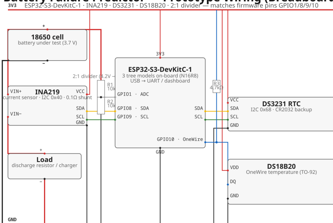
Fig. 1. Prototype wiring for the ESP32-S3 deployment. The battery discharges through the INA219 shunt into a load, the 2:1 divider senses cell voltage at ADC GPIO1, and I2C (GPIO8/9) serves the INA219 and DS3231 while OneWire (GPIO10) reads the DS18B20. The boards are a $12 ESP32-S3-DevKitC-1 and two breakout modules.
