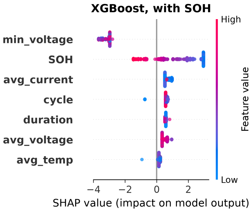
FIGURE 6. SHAP feature importance for XGBoost in NASA-to-Oxford transfer at H=20, with SOH. SOH dominates by a wide margin.
