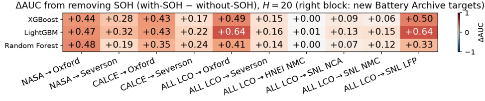
Figure 2: Transferability collapse map at H=20 for the tree ensembles: the AUC drop from removing SOH, per source→target pair and model. Positive values mean SOH removal destroys apparent transfer performance; the near-uniform saturation at the maximum drop is the signature of a single-feature shortcut rather than of distributed degradation knowledge. Right block: ALL-LCO → new Battery Archive targets. GRU deltas are reported in the text.
