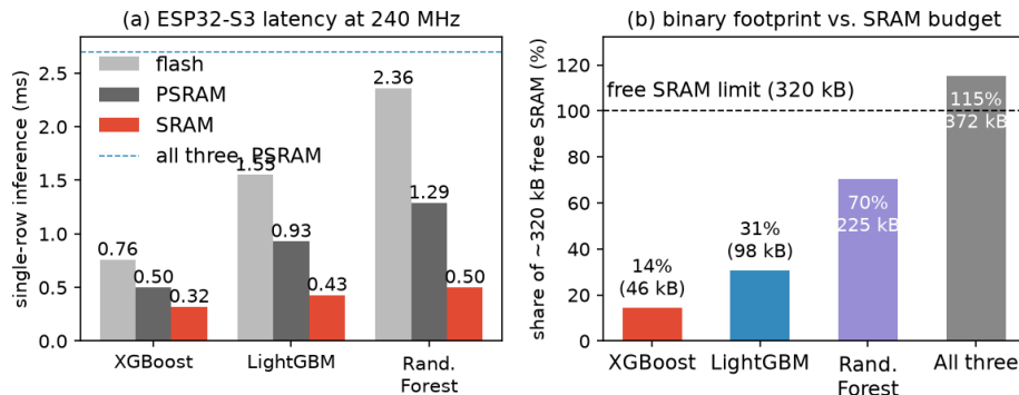
Figure 3: Deployment trade-offs: (a) measured single-row inference time per model at 240 MHz with the binary in memory-mapped flash, PSRAM, or a single model in internal SRAM (dashed line: all three models from PSRAM); (b) per-model and combined binary footprint as a share of the ESP32-S3’s roughly 320 kB of free internal SRAM — each model fits, the combined 372 kB binary does not.
