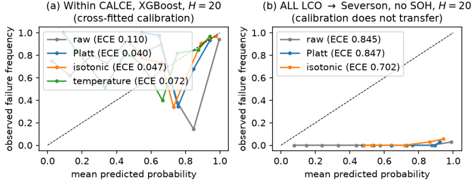
Figure 1: Reliability diagrams under the cross-fitted protocol. (a) Within CALCE, XGBoost at H=20 : the fitted Platt sigmoid preserves ranking but washes confidence toward the base rate. (b) ALL-LCO → Severson without SOH at H=20 : no fitted calibrator, whichever source scores it is applied to, repairs calibration on the shifted target.
