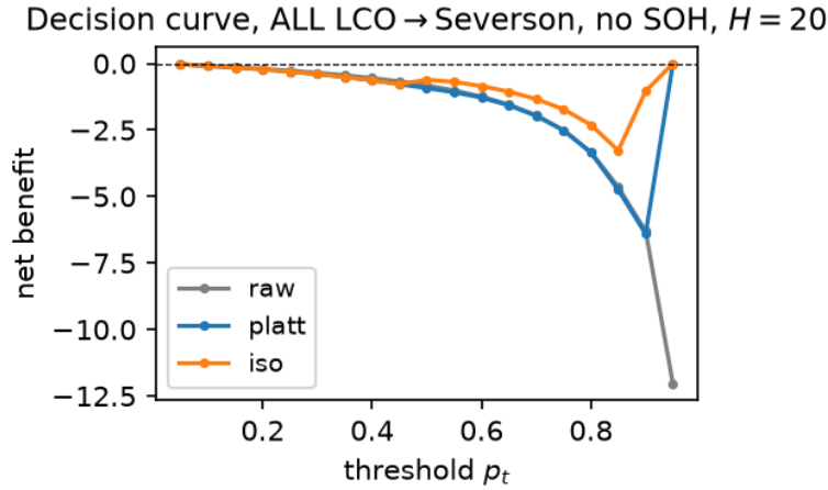
Figure 3: Decision-curve analysis (net benefit vs. threshold) for ALL-LCO → Severson without SOH at H=20 : no score type produces a usable operating point once SOH is removed.
