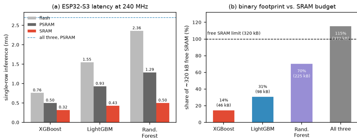
FIGURE 13. Deployment trade-offs: (a) measured single-row inference time per model at 240 MHz with the binary in memory-mapped flash, PSRAM, or a single model in internal SRAM (dashed line: all three models from PSRAM); (b) per-model and combined binary footprint as a share of the ESP32-S3's roughly 320 kB of free internal SRAM – each model fits, the combined 372 kB binary does not.
