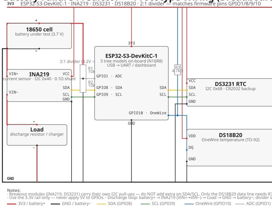
FIGURE 1. Prototype wiring for the ESP32-S3 deployment. The battery discharges through the INA219 shunt into a load, the 2:1 divider senses cell voltage at ADC GPIO1, and I2C (GPIO8/9) serves the INA219 and DS3231 while OneWire (GPIO10) reads the DS18B20. The boards are a $12 ESP32-S3-DevKitC-1 and two breakout modules.
