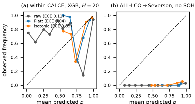
Fig. 3. Reliability diagrams under the cross-fitted protocol. (a) Within CALCE (XGBoost, H=20 ). (b) ALL-LCO→Severson without SOH ( H=20 ): no source-fitted calibrator lands near the diagonal on the shifted target.
