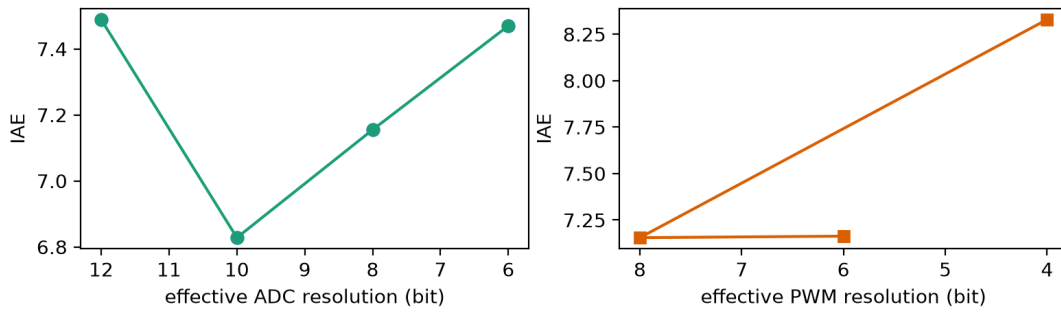
Fig. 6. Effective-resolution sweep at the N=64 achievable schedule. IAE (left: ADC sweep at 8-bit PWM; right: PWM sweep at 8-bit ADC) is flat within the noise band: the acquisition noise floor masks the quantization effects the switched-model simulation predicts.
