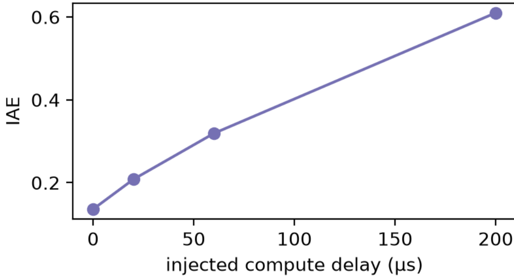
Fig. 8. Injected computational latency at the fast schedule: effective period grows 73 to 274 \mu\text{s} and IAE by 4.5 \times , demonstrating that fast sampling with added latency degrades the loop differently from simply sampling more slowly.
