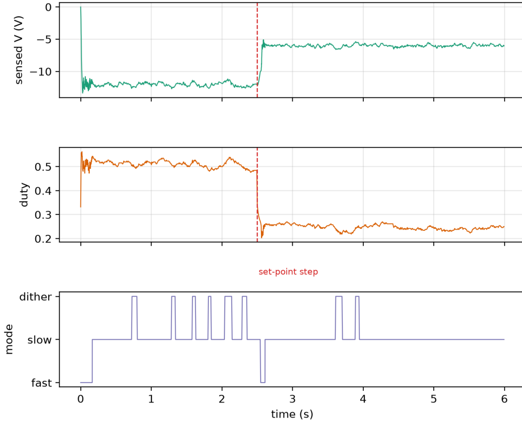
Fig. 9. Adaptive schedule+dithering run on the ESP32-S3 ( N=8 fast, N=64 slow). Top: sensed output with a set-point step from -12 to -6 V at 2.5 s (dashed). Middle: duty. Bottom: selected mode. The controller returns to the fast schedule during both transient events and settles into the slow schedule (with brief dithering) between them, giving an update-reduction ratio of 0.84 .
