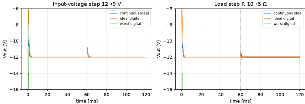
FIGURE 7. Disturbance response: 2%-settling trajectories for input step V_{\text{in}} : 12 \rightarrow 9 V and load step R : 10 \rightarrow 5 \Omega at t = 60 ms on the continuous baseline, ideal digital controller, and the worst combined configuration (5 \times , 8-bit ADC, 12-bit PWM).
