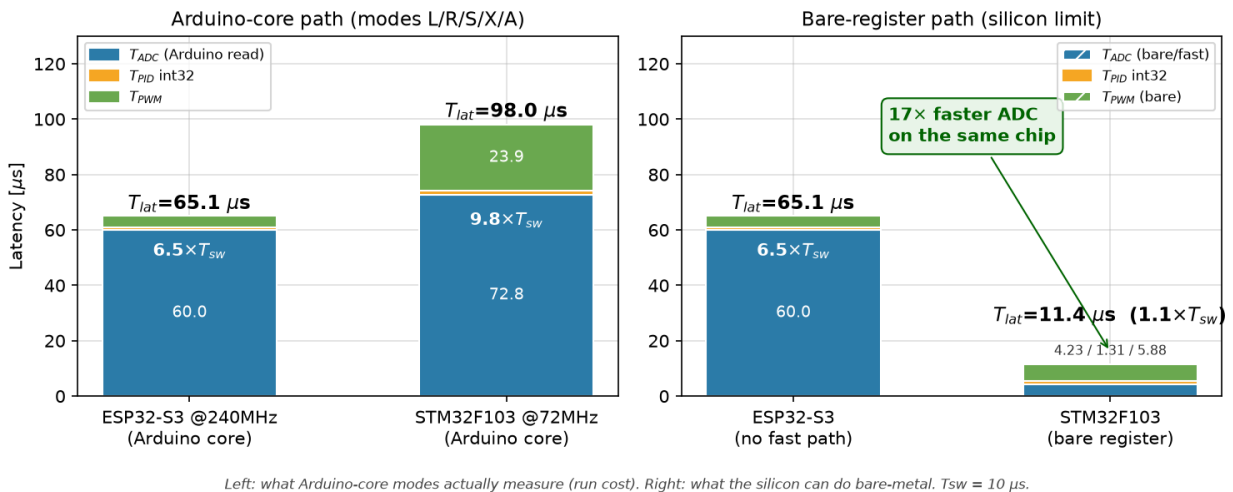
FIGURE 14. Cross-platform latency: Arduino-core path vs bare-register path. Left: what the deployed modes measure; right: what the silicon can do. The STM32F103 ADC is 17× faster bare-metal on the same chip.
