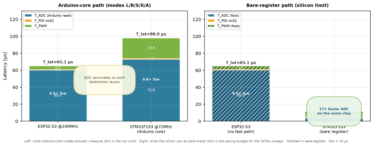
FIGURE 14. Cross-platform latency: Arduino-core path vs bare-register path. Left: what the deployed modes measure; right: what the silicon can do. The STM32F103 ADC is 17\times faster bare-metal on the same chip.
