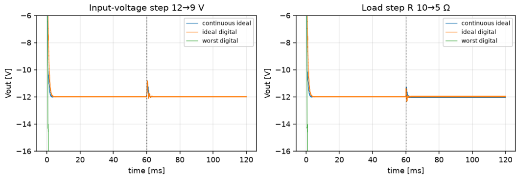
FIGURE 7. Disturbance response: 2%-settling trajectories for input step V_{\text{in}} : 12 \rightarrow 9\text{ V} and load step R : 10 \rightarrow 5\text{ }\Omega at t = 60\text{ ms} on the continuous baseline, ideal digital controller, and the worst combined configuration (5×, 8-bit ADC, 12-bit PWM).
