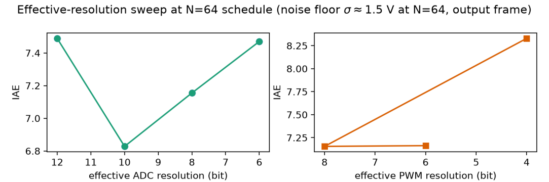
FIGURE 10. Effective-resolution sweep at the N=64 achievable schedule. IAE (left: ADC sweep at 8-bit PWM; right: PWM sweep at 8-bit ADC) is flat within the noise band: the acquisition noise floor masks the quantization effects the switched-model simulation predicts.
