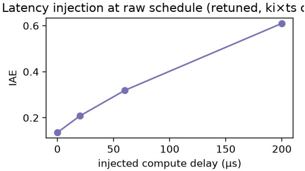
FIGURE 12. Injected computational latency at the fast schedule: effective period grows 73 to 274 \mu\text{s} and IAE by 4.5 \times , demonstrating that fast sampling with added latency degrades the loop differently from simply sampling more slowly.
