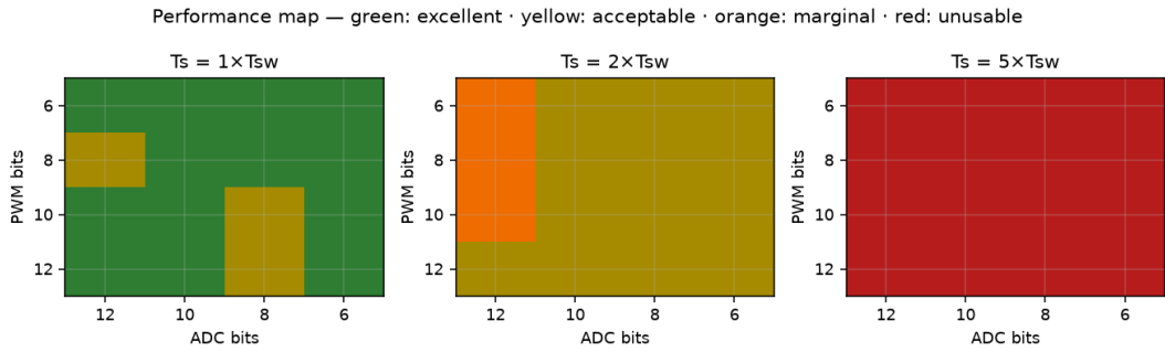
FIGURE 6. Performance map of the 48-run sweep. Thresholds: excellent ( t_{\text{settle}} \leq 4\text{ ms} , |e_{\text{ss}}| \leq 60\text{ mV} , \text{LC} \leq 60\text{ mV} , \text{ov} \leq 5\% ), acceptable ( t_{\text{settle}} \leq 6\text{ ms} , |e_{\text{ss}}|, \text{LC} \leq 120\text{ mV} ), marginal, unusable ( t_{\text{settle}} \geq 50\text{ ms} ).
