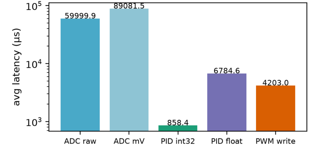
Measured control-loop latency breakdown (ESP32-S3, 24
