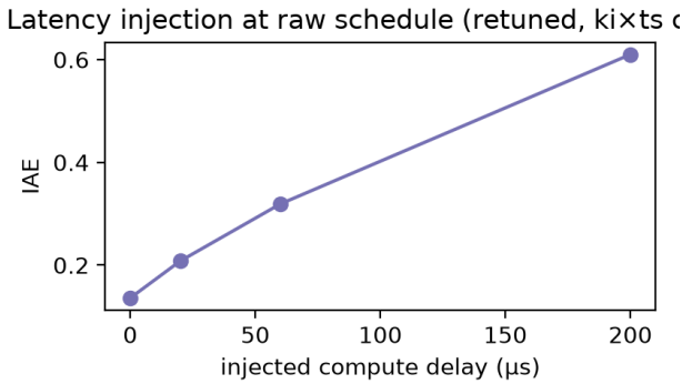
FIGURE 11. Injected computational latency at the fast schedule: effective period grows 73 to 274 \mu\text{s} and IAE by 4.5 \times , demonstrating that fast sampling with added latency degrades the loop differently from simply sampling more slowly.
