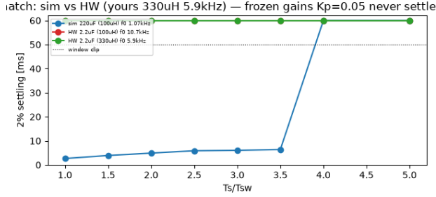
FIGURE 21. LC mismatch bound (frozen gains, 60 ms window): simulated 220\mu\text{F} ( 1.07\text{ kHz} , blue) settles to 3.5\times then fails at 4\times ; HW 2.2\mu\text{F} with 100\mu\text{H} ( 10.7\text{ kHz} , red) and as-wired 330\mu\text{H} ( 5.9\text{ kHz} , green) never settle even at 1\times (59.9 ms window-clip). The 35\text{--}40\mu\text{s} boundary does not transfer to the LC plant without retuning; see §V-G for the wired 330\mu\text{H} hardware that does settle with averaged reads.
