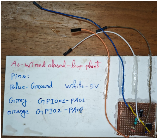
FIGURE 9. As-wired protoboard as tested ( 330\ \mu\text{H} , 2.2\ \mu\text{F} , LM358, 5'). Pinout handwritten on board: Blue—GND, White—5V, Grey—GPIO1/PA1 (ADC), Orange—GPIO2/PA8 (PWM). The same board was used for ESP32-S3 (GPIO1/2) and STM32F103 (PA1/PA8) captures in §V-G, Table 6 and Table 7 (photo: Hardware/testedcircuit.jpeg).
