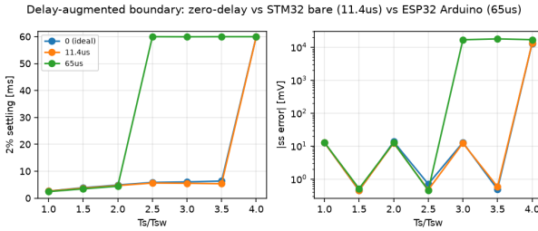
FIGURE 18. Delay-augmented boundary sweep (16-bit, 60 ms window). Zero-delay (blue) loses regulation at 4 \times ; 11.4 \mu s (STM32 bare, orange) similar; 65 \mu s (ESP32 Arduino, green) loses at 2.5 \times ( T_s + T_{lat} \approx 90 \mu s). Markers at 59.9 ms are window-clip “never settled”.
