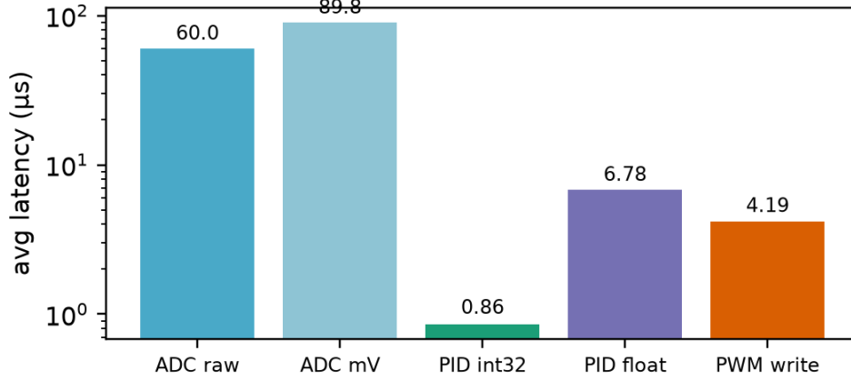
FIGURE 10. Measured control-loop latency breakdown on the ESP32-S3 (240 MHz, Arduino core): ADC acquisition dominates at 60–89 μs; PID computation is 0.86 μs (int32) to 6.8 μs (float32); PWM register write is 4.2 μs. Log scale.
