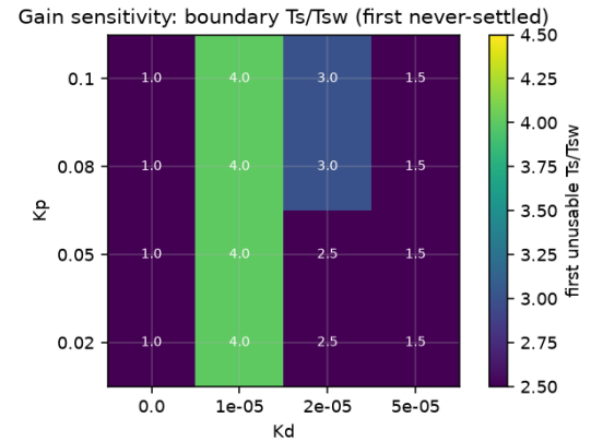
FIGURE 20. Gain sensitivity: first unusable T_s/T_{sw} (window-clip) vs K_p/K_d . K_d = 10^{-5} (paper) is the ridge ( 4 \times across K_p ); boundary moves \leq 1.5 \times only via K_d .
