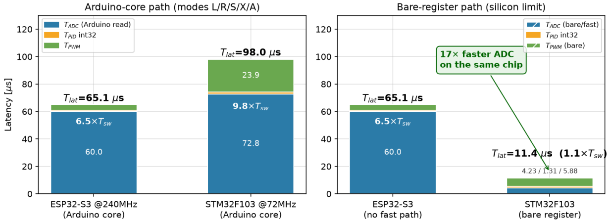
FIGURE 15. Cross-platform latency: Arduino-core path vs bare-register path. Left: what the deployed modes measure; right: what the silicon can do. The STM32F103 ADC is 17\times faster bare-metal on the same chip.
