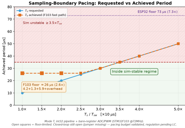
FIGURE 17. Mode T sampling-boundary pacing (STM32F103 @72 MHz, int32 + bare-register). Open squares are floor-limited. The ESP32-S3 floor (73 \mu s, 7.3 \times T_{sw} ) lies above the entire sweep; the STM32F103 bare path paces through the predicted 3.5 \times T_{sw} boundary. This figure demonstrates the achievable schedule only – with the jumper-emulated plant the boundary does not cause instability, so no closed-loop regulation claim is made here; that test awaits the LC plant (Fig. 8).
