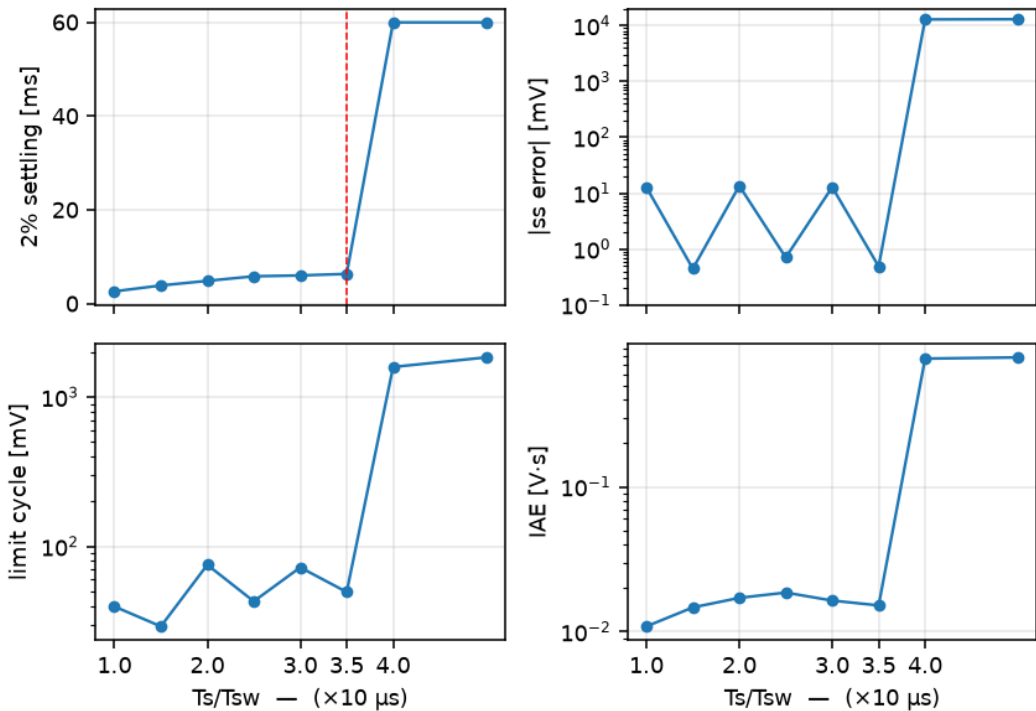
FIGURE 3. Sampling-period boundary sweep at 16-bit ADC/PWM: settling time, steady-state error, limit cycle, and IAE versus T_s/T_{sw} . Regulation is lost between 3.5\times and 4\times T_{sw} .
