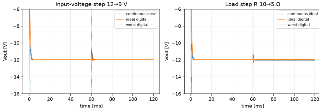
FIGURE 7. Disturbance response: 2%-settling trajectories for input step V_{\text{in}} : 12 \rightarrow 9 V and load step R : 10 \rightarrow 5 \Omega at t = 60 ms on the continuous baseline, ideal digital controller, and the worst combined configuration (5 \times , 8-bit ADC, 12-bit PWM).
